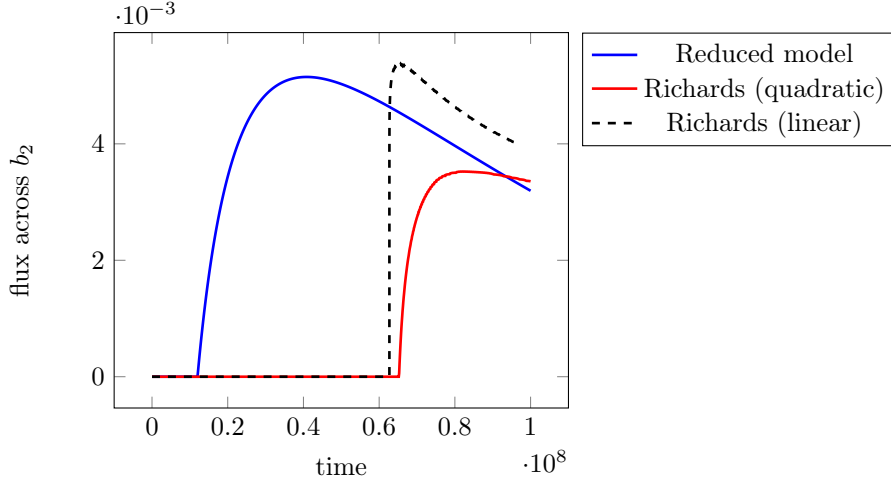
FIGURE 6. Flux across the first interface b_2 located at z = 1500m starting from the bottom computed with the reduced model (blue solid line), with Richards equation with quadratic relative permeabilities (red solid line), and with Richards equation with linear relative permeabilities (dashed black line).
