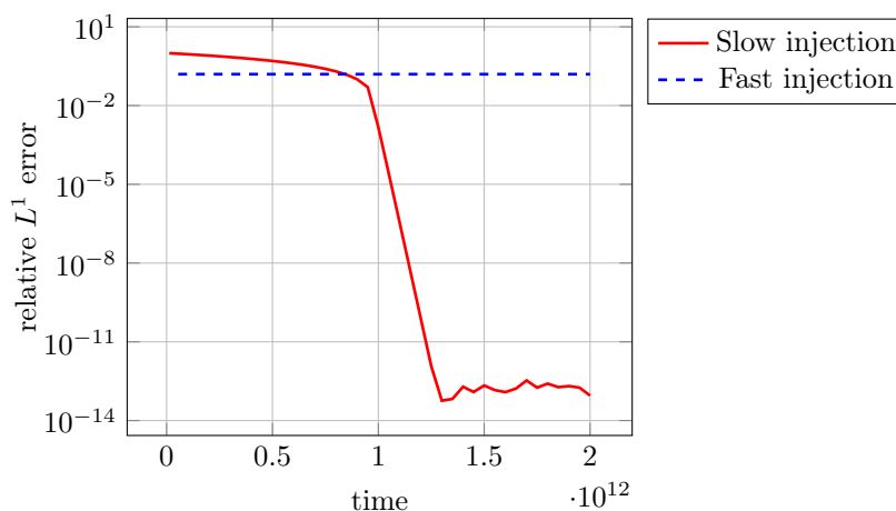
FIGURE 12. Evolution of the relative L^1 distance between the solution given by our model and the one given by the ray-tracing algorithm.
