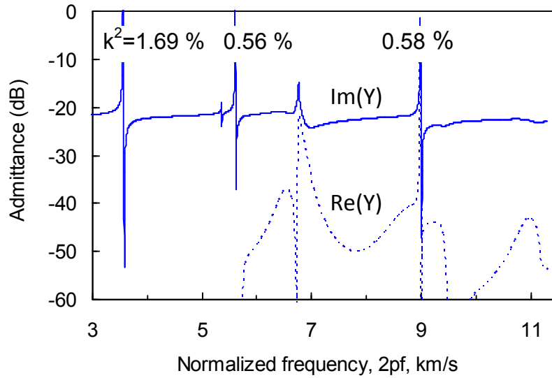
Fig. 6. Real and imaginary parts of admittance obtained numerically for \text{Sc}_{0.4}\text{Al}_{0.6}\text{N}/\text{Sapphire} with Cu grating. The thicknesses of ScAlN film and Cu electrodes are h_f=0.515 \lambda , and h_{\text{Cu}}=0.05 \lambda , respectively.
