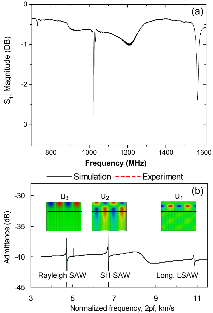
Fig. 3 (a) Experimental response of SAW resonators based on \text{Sc}_{0.09}\text{Al}_{0.91}\text{N}/\text{Sapphire} structure (b) Simulated admittance of Al grating on \text{Sc}_{0.09}\text{Al}_{0.91}\text{N}/\text{Sapphire} obtained with fitted constants, compared with experimental velocity values. The thicknesses of ScAlN and Al electrodes are h_{\text{ScAlN}}=0.425\lambda , and h_{\text{Al}}=0.023\lambda , respectively.
