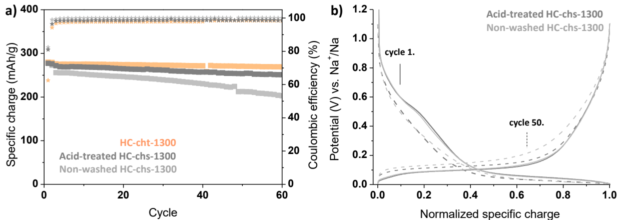
Figure 8 (a) Specific charge (squares) and Coulombic efficiency (stars) of the Na-ion half-cells tested with electrodes based on chitin- and chitosan-derived HCs. For clarity, only the specific charge obtained during charge (desodiation) is presented in the graph. (b) Evolution of the polarization during 1 st and 50 th cycle for the cells assembled with the electrodes based on non-washed and acid-treated HC-chs-1300.
