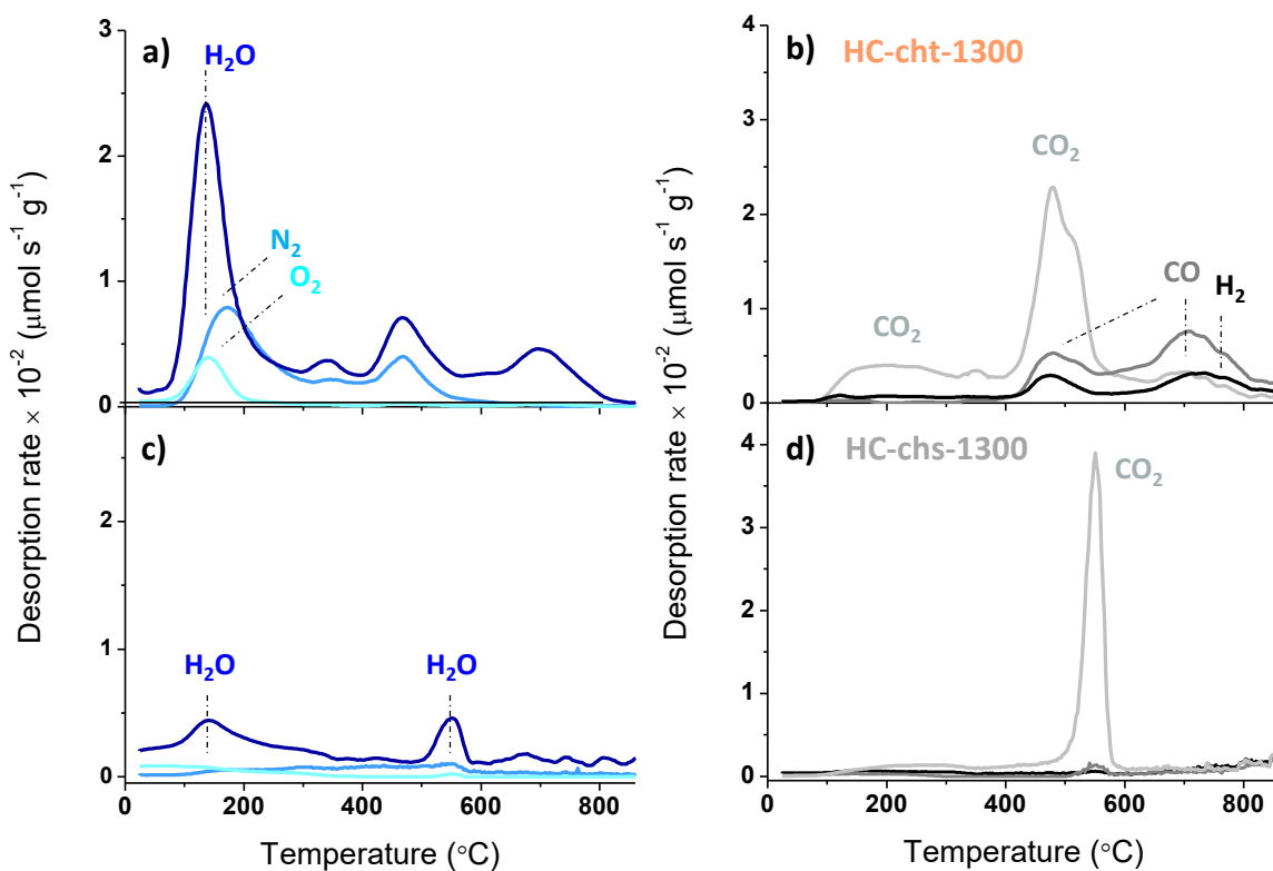
Figure 6 TPD-MS spectra collected for (a, b) chitin- and (c, d) chitosan-derived HCs. For clarity the spectrum of each HC was split into two graphs: (a and c) one showing only the evolution of H 2 O, N 2 , and O 2 , and (b and d) the second graph presenting the desorption profiles of CO 2 and other detected gases.
