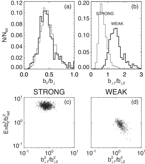
Figure 3. Top panels: distribution in the strong- and weak-expansion data sets (thin and thick lines, respectively) of the ratio between the amplitude of field-parallel and field-perpendicular magnetic fluctuations, b_{\parallel}/b_{\perp 1} (left) and of the amplitudes of magnetic fluctuations in the two field-perpendicular components, b_{\perp 1}/b_{\perp 2} (right). Bottom panels: scatterplot of b_{\perp 1}^2/b_{\perp 2}^2 versus E = b_{\perp 1}^2/b_{\perp 2}^2 for the strong- and weak-expansion data sets in the bottom left and bottom right panels, respectively.
