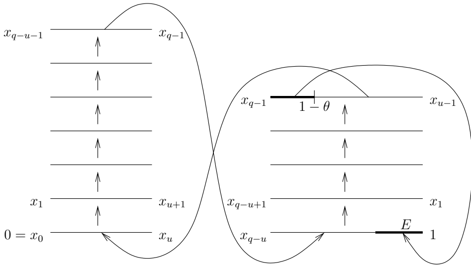
Figure 2: Behaviour of T_\theta on the intervals I_0, \dots, I_{q-1} when \theta < p/q .
