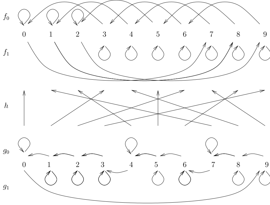
Figure 3: The maps f_0, f_1, h, g_0, g_1 when p = 3 and q = 10 , so u = 7, v = 2 and L = \{0, 4, 7\} .
