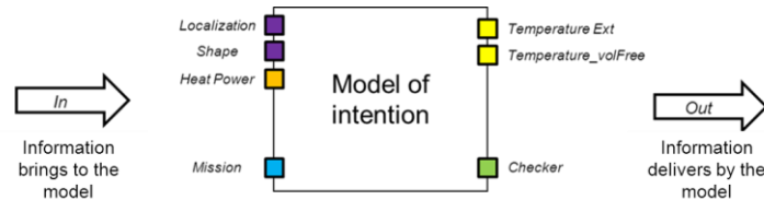
Figure 4: A blank model of intention with different port type (color) associated to attributes (name)
