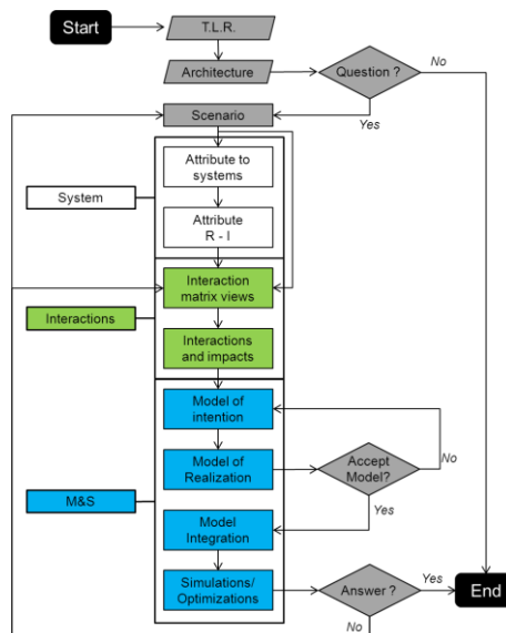
Figure 2: Global methodology
