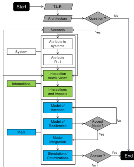
Figure 2: Global methodology
