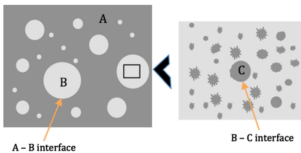
Figure 2 Schematic of immiscibility within calcium borosilicate glasses [47]. The residual phase A is rich in Si, while heterogeneously distributed deposits of varying size called phase B are rich in Ca (and Mo). Within these phase B regions, there are additional deposits with varying geometry that are designated as phase C and are compositionally a mixture of phases A and B.
