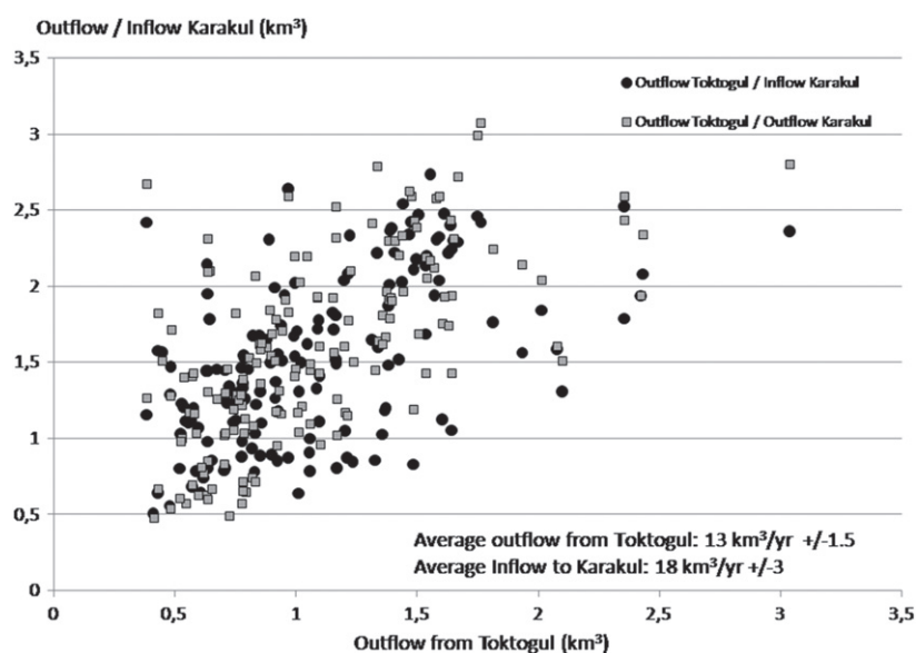
Figure 4. Scatter plot of monthly water inflow volumes and outflow volumes of the Karakul with respect to outflow from the Toktogul reservoirs (monthly data from the Cawater database).
