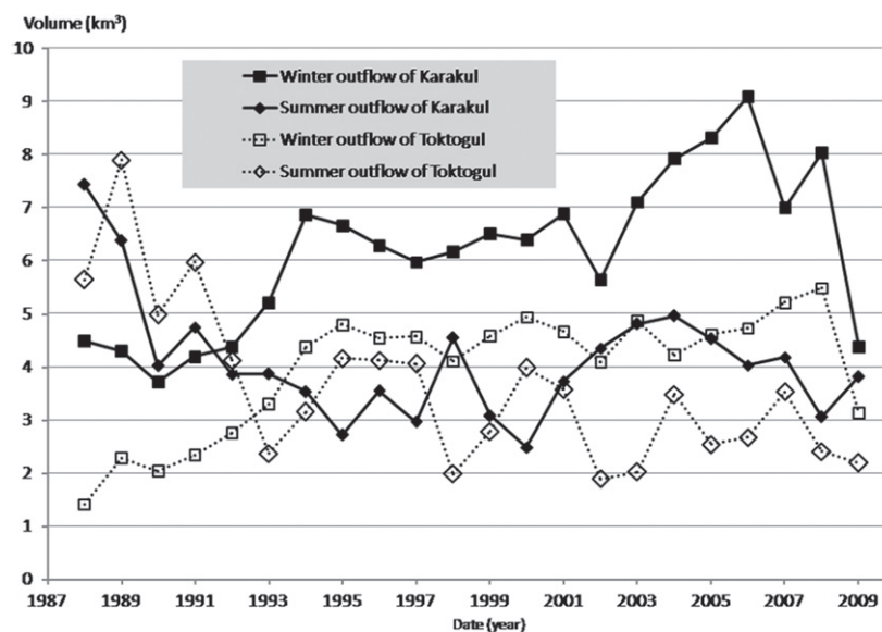
Figure 3. Monthly water outflow volumes in winter (January–March) and in summer (June–August) for the Toktogul and the Karakul reservoirs. The data have been downloaded from the Cawater database ( www.cawater-info.net ).
