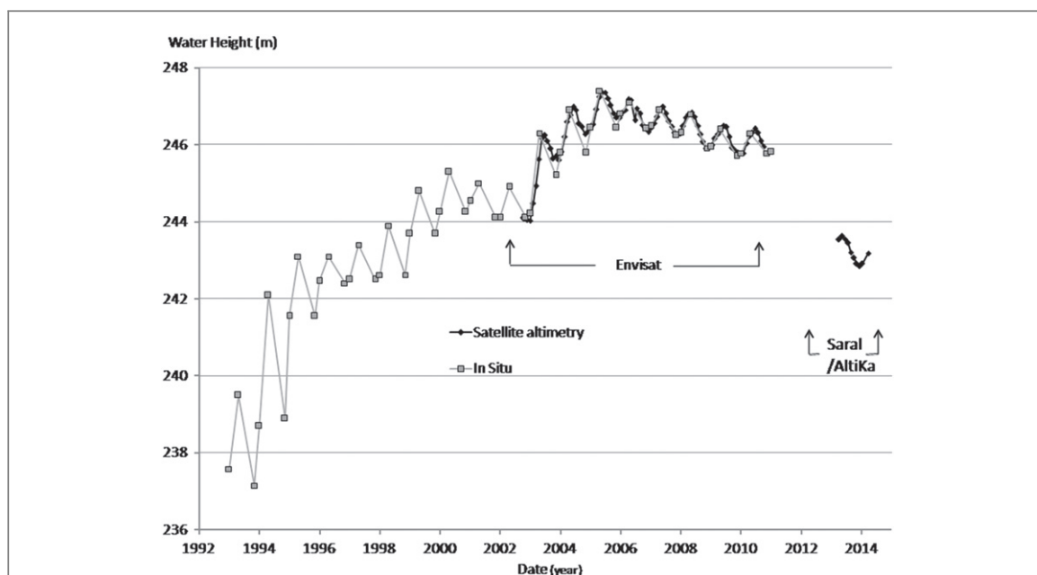
Figure 6. Water height variations of the Lake Aydarkul, inferred from radar altimetry measurements on ENVISAT and SARAL/AltiKa altimeters (dates of measurements are the average dates of the four passes every 35 days) and from in situ at the dates of minimum and maximum level of each year (downloaded from the Cawater database).
