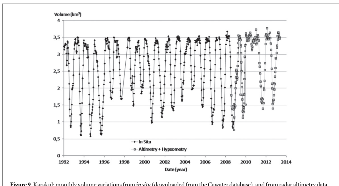
Figure 9. Karakul: monthly volume variations from in situ (downloaded from the Cawater database), and from radar altimetry data using the relationship: (V = 0.014\ 73\ L^2 - 9.73L + 1606.1) .
