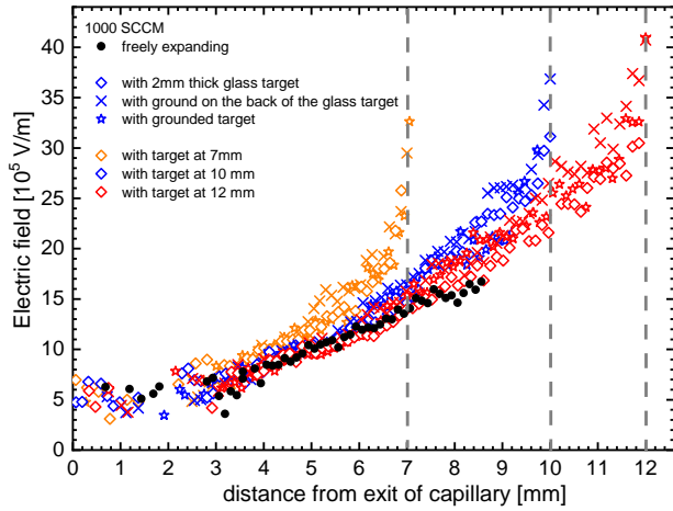
Figure 6. Electric field profiles as a function of the distance from the exit of the capillary. The measurements were taken at 30 kHz, 2 kV amplitude (4 kV pp ). Three different targets were used (glass, glass with a metallic layer at the back side and grounded metal) at distances of 7 mm, 10 mm and 12 mm from the exit of the capillary at a single He flow of 1000 SCCM. The positions of the targets are indicated by dashed lines. Error bars were omitted for better readability of the graph. Like in other graphs, the error bars are the largest very close to the capillary, where the electric field is the lowest, and just next to the surface of the target.
