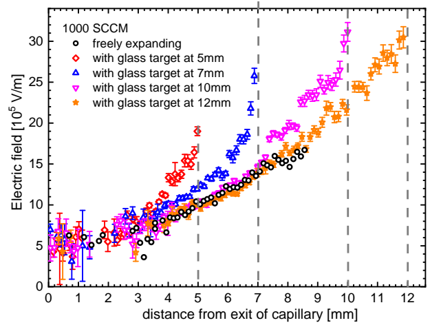
Figure 5. Electric field profiles as a function of the distance from the exit of the capillary. The measurements were taken at 30 kHz, 2 kV amplitude (4 kV pp ). Glass target at different distances was used (5 mm, 7 mm, 10 mm and 12 mm) at a single He flow of 1000 SCCM. The positions of the targets are indicated by dashed lines.
