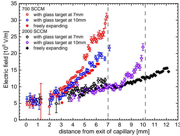
Figure 4. Electric field profiles as a function of the distance from the exit of the capillary. The measurements were taken at 30 kHz, 2 kV amplitude (4 kV pp ). Glass target was used at 7 mm and 10 mm for He flows at 700 SCCM and 2000 SCCM. The positions of the targets are indicated by dashed lines.
