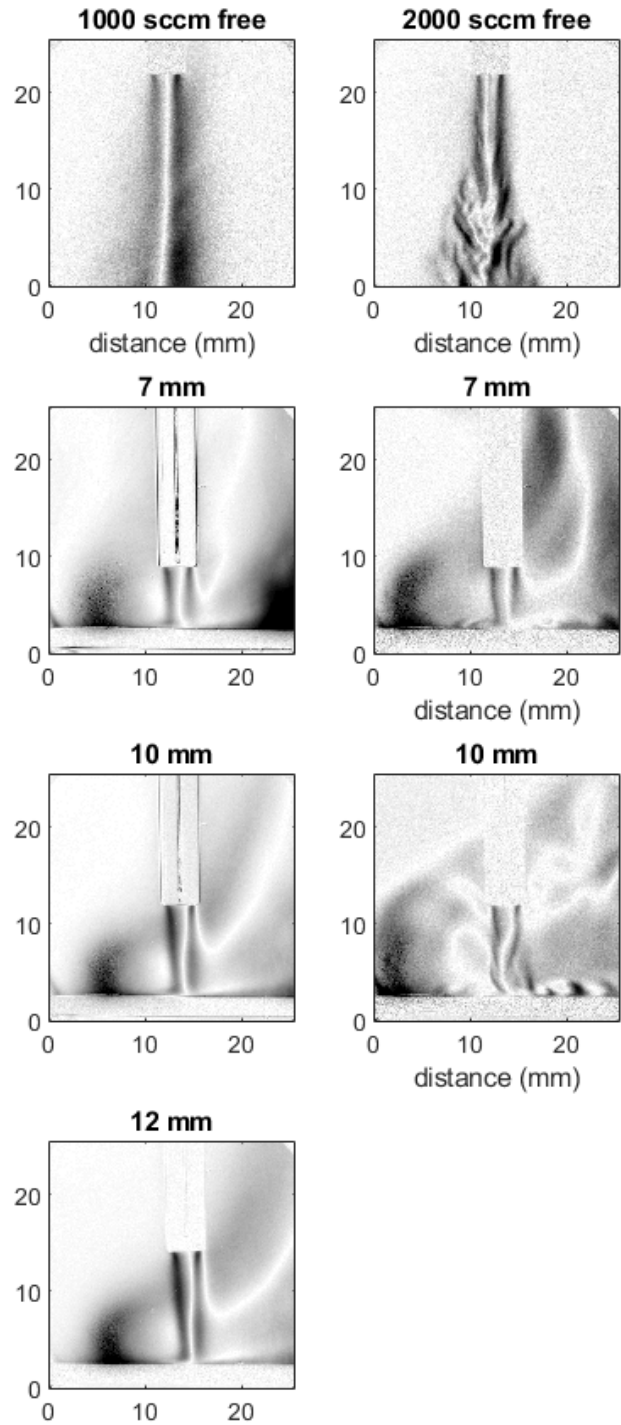
Figure 7. The visualization of the flow for two different flow speeds (1000 SCCM and 2000 SCCM) in a freely expanding jet and with a glass target at different distances. Flow visualization of freely expanding jets was shown in [26].
