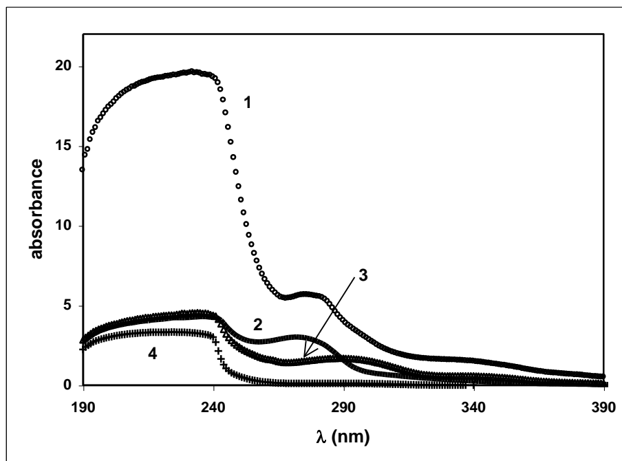
Figure 1: Absorption spectra of BumimPF 6 of various origin. (1): raw BumimPF 6 -SI ; (2): raw BumimPF 6 , (Cl - ) = 46 \pm 5 ppm ; (3): purified BumimPF 6 -SI ; (4): purified BumimPF 6 .
