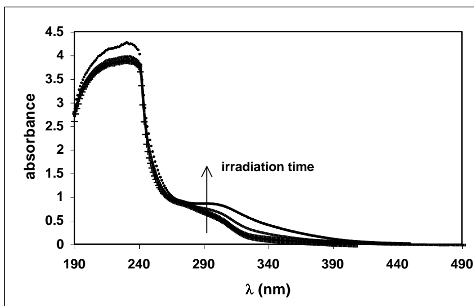
Figure 3: Absorption spectra of raw BumimPF 6 (with (Cl - ) ≈ 46 ppm) after various time of pulse laser irradiation. Average laser power 13 mW, repetition rate 10 Hz, \lambda_{\text{exc}} = 266 nm, t_{\text{irr}} = 0 min, 56 min and 93 min.
