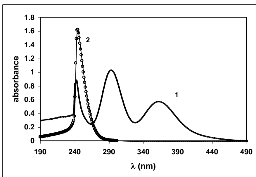
Figure 5: Absorption spectrum of: (1) EuI 2 ( C = 10^{-4} M) in BumimPF 6 and (2) KI ( C = 2.4 \times 10^{-3} M) in BumimPF 6 .
