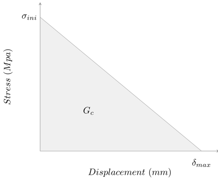
Figure 3: Cohesive behaviour with the stress as a function of the opening of the crack.
