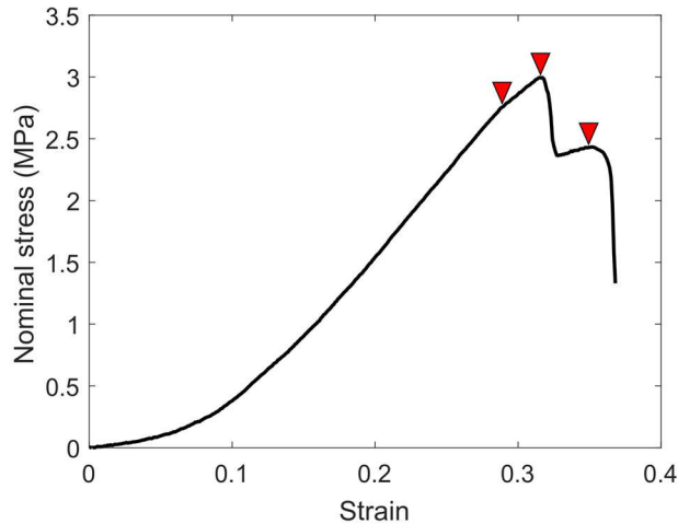
Figure 4: Example of experimental stress-strain curve, with manually selected damage initiation points (red arrow).
