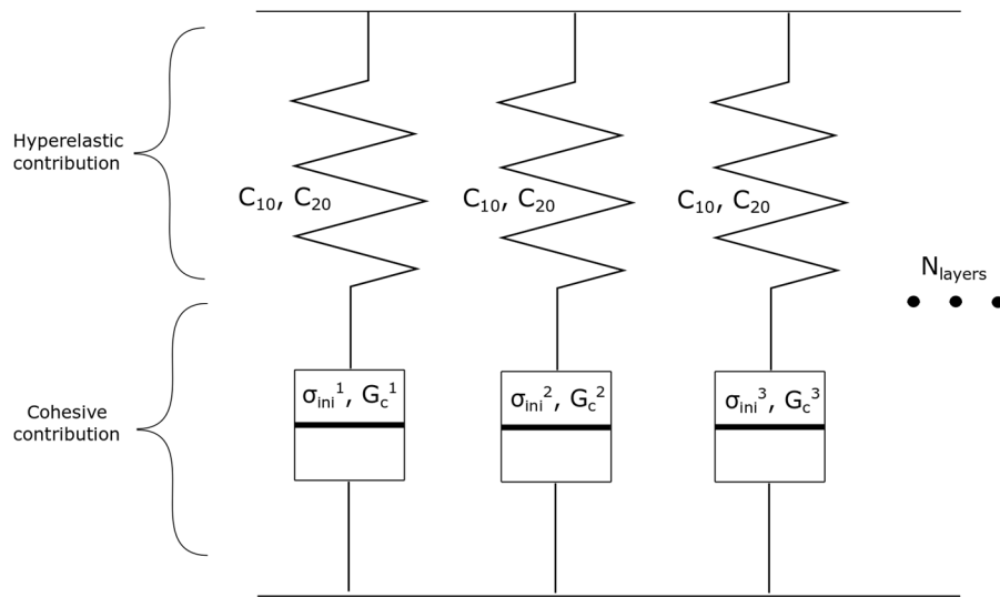
Figure 2: Schematic representing the analytical model and its material parameters.
