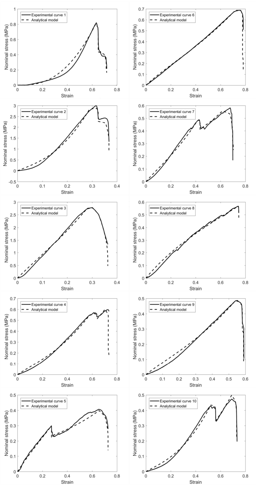
Figure 6: Comparison between the analytical model (dashed curve) and the experimental tensile test (solid curve). The r^2 are in a range of 0.97 to 0.99
