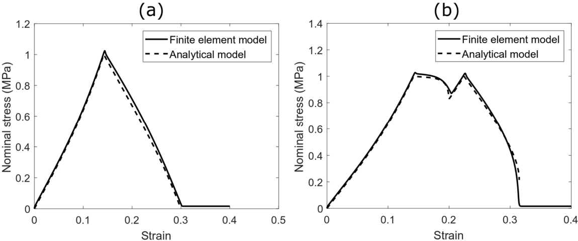
Figure 5: Responses of analytical model (dashed curve) and finite element model (solid curve) with (a) one layer and (b) two layers, with the two peaks corresponding to each layers damaging successively.
