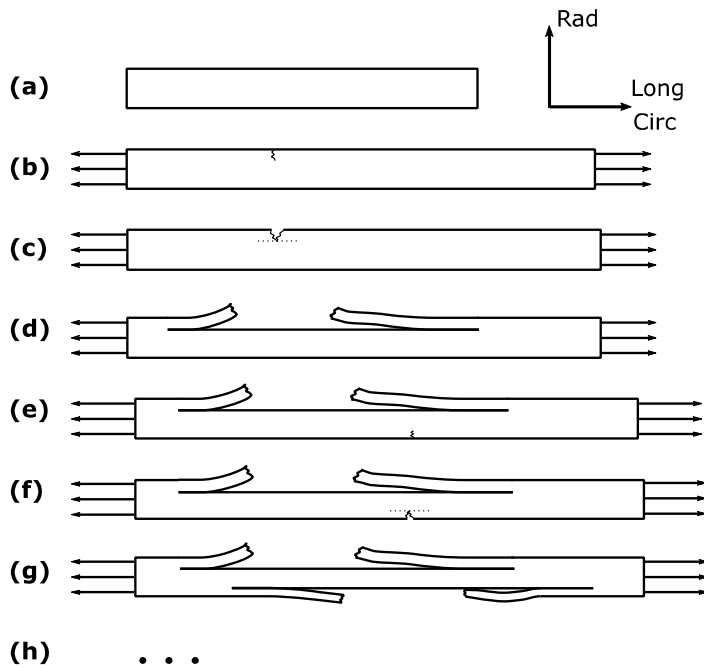
Figure 1: schematic representation of the damage initiation and propagation mechanism observed in situ . (a) intact sample, (b and c) initial radial crack, opening in mode I, (d) elastic recoil of the ruptured layers, causing a mode II longitudinal crack to form and propagate, (f, g, h...) the process repeats until complete failure of the sample. Modified from Helfenstein-Didier et al. [6].
