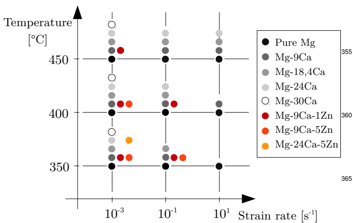
Figure 12: Formability of alloys as a function of temperature and strain rate.
