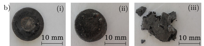
Figure 7: a) Influence of Zn at 400 \text{ °C}/10^{-3} \text{ s}^{-1} ; b) Specimens after compression at 400 \text{ °C}/10^{-1} \text{ s}^{-1} at \epsilon=2 : (i) Mg-9Ca, (ii) Mg-9Ca-1Zn and (iii) Mg-9Ca-5Zn.
