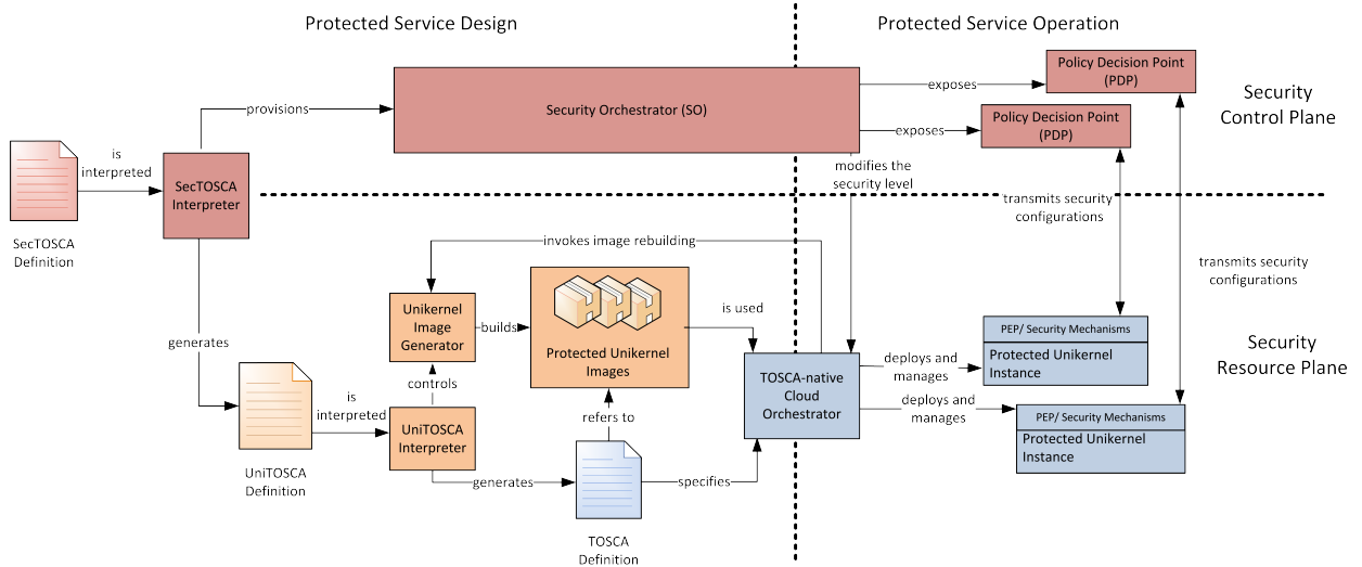
Figure 5. Overview of the TOSCA-oriented software-defined security framework for protecting cloud services.
