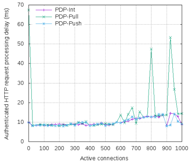
Figure 9. Authenticated HTTP processing time with the different approaches.
