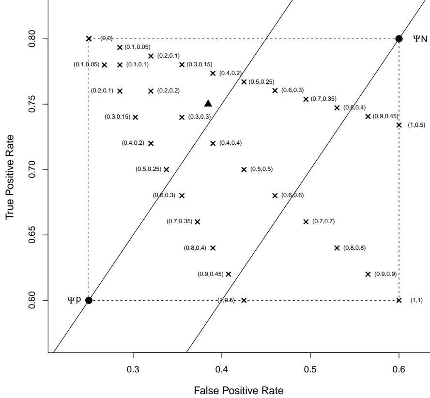
Figure 8: Visualization of the classification cost of a reject classifier in the ROC space with ratios (\frac{\lambda_{RP}}{\lambda_{FN}}, \frac{\lambda_{RN}}{\lambda_{FP}}) .
