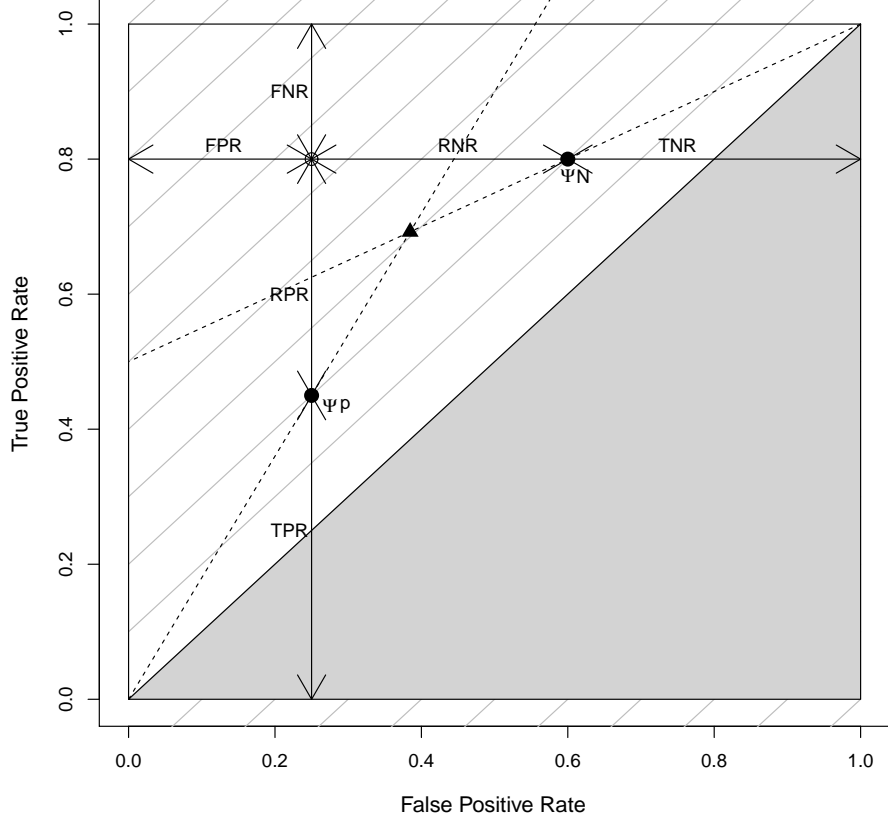
Figure 7: Visualisation of a reject classifier in the ROC space.
