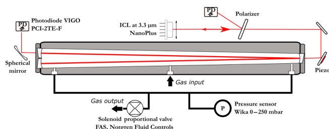
Figure 1. Details of the optical setup with the laser injection and phase control (piezo mounted on the injection steering mirror assembly). The polarizer is tilted and its reflection used for acquiring the laser power spectrum before the cavity injection. At the cavity output, a spherical mirror is used to focus the light on the second (signal output) photodiode.
