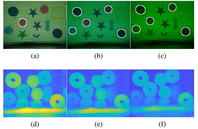
Fig. 12. (a) Image f_\Gamma acquired with a small concentration, \Gamma , of colourant. The probe function b is delineated in white. (b) Ball detection in an image f_{3\Gamma} acquired with an intermediate concentration, 3\Gamma , of colourant. (c) Ball detection in an image f_{12\Gamma} acquired with a high concentration – 12\Gamma – of colourant. (d) Map of LIP-multiplicative Asplund distances Asp_{bc,p}^\Delta f_\Gamma^c of the image f_\Gamma . (e) Map Asp_{bc,p}^\Delta f_{3\Gamma}^c of the image f_{3\Gamma} . (f) Map Asp_{bc,p}^\Delta f_{12\Gamma}^c of the image f_{12\Gamma} . The tolerance parameter p is set to 90%.
