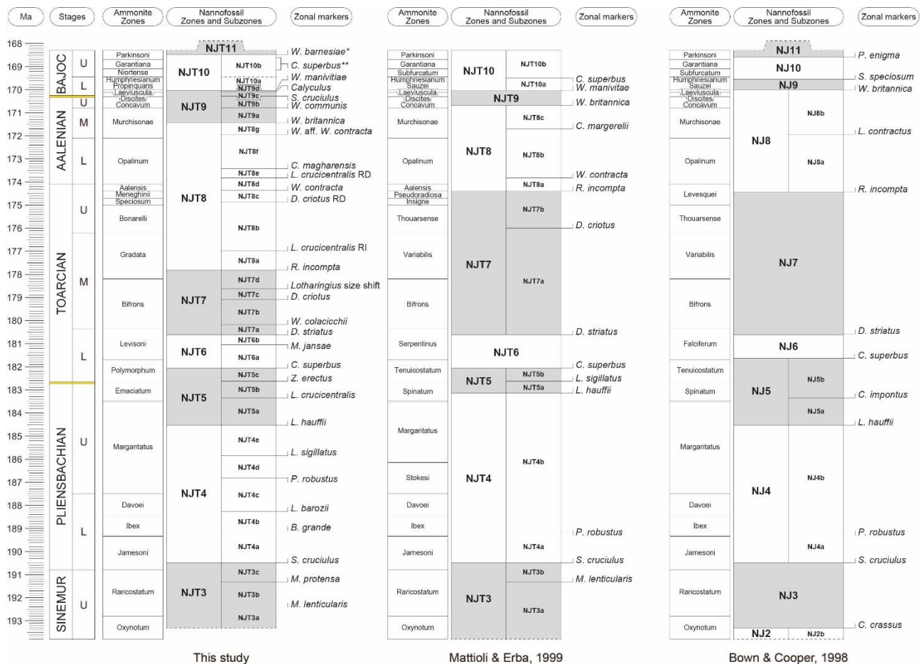
Figure 3. Nannofossil zonation defined for the Lusitanian Basin and its comparison with existing biozonation schemes covering the same time interval. Geochronology and ammonite zone durations after Gradstein et al. (2012), and ammonite biohorizons position have an error of ~100 kyr. (*) bioevent recorded by López-Otálvaro and Henriques (2018) in Cabo Mondego; (**) indicate the age interval where is predictable to observe the LO of Carinolithus superbus . The ammonite zonal markers used in Central Italy (Mattioli and Erba, 1999) and NW Europe (Bown and Cooper, 1998) are sometimes different from the Lusitanian Basin. Some discrepancies between zonal boundaries may occur in the different localities. See the text for more explanation.
