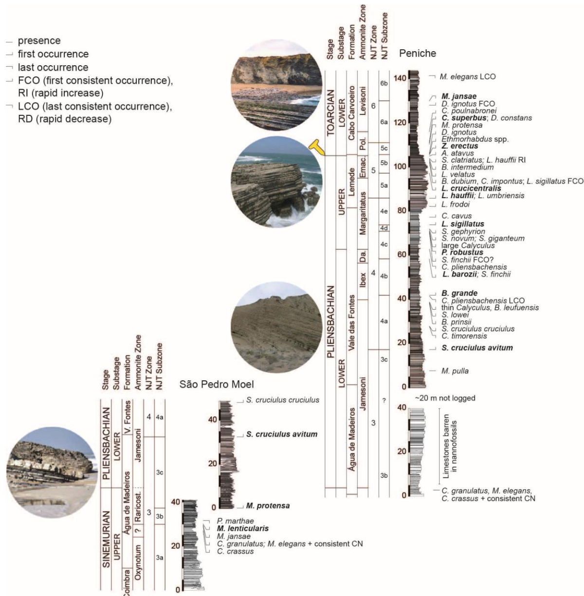
Figure 2. Composite log of the five studied sections where ~100 nannofossil bioevents (FO, LO, FCO, LCO, RI, RD) recorded in ~24 Myr time span are plotted. Lithostratigraphy and ammonite biostratigraphy from Mouterde et al. (1955), Duarte and Soares (2002), Azerêdo et al. (2003) and Duarte et al. (2014). (a) Composite log of S. Pedro de Moel and Peniche sections. Raricos. = Raricostatum; Dav. = Davoei; Emac. = Emaciatum; Poly. = Polymorphum. Consistent CN: levels in which the record of calcareous nannofossils becomes consistent. (b) Composite log of Rabaçal, Brenha and Cabo Mondego sections. Poly. = Polymorphum; Bona. = Bonarelli; Specio. = Speciosum; Men. = Meneghinii; Aal. = Aalensis; Conca. = Concavum; Dis. = Discites; Hu. = Humphriesianum.
