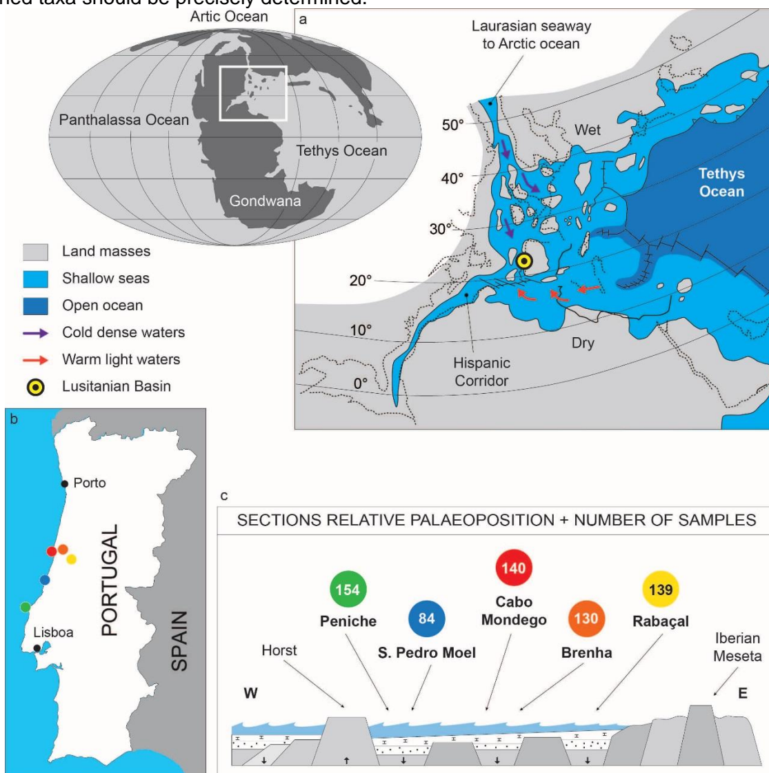
Figure 1. (a) Western Tethys palaeogeography and location of the Lusitanian Basin within the proto-Atlantic rift during the Toarcian (modified after Bassoulet et al., 1993). (b) Location of the five studied sections in west Portugal, (c) their relative cross-section palaeoposition and the number of samples studied in each one of them.
