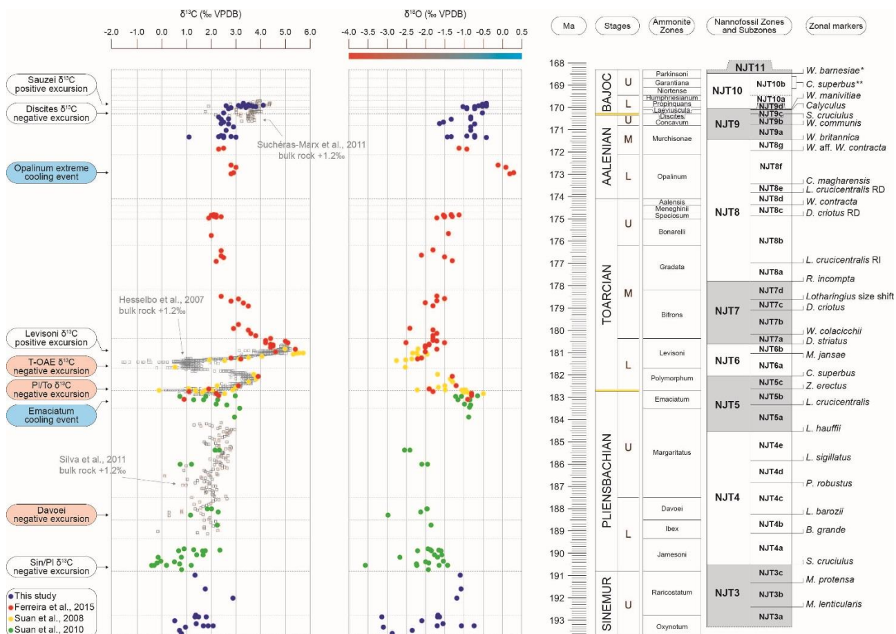
Figure 4 - Nannofossil zonation scheme and \delta^{13}\text{C}_{\text{brachiopod}} plus \delta^{18}\text{O}_{\text{brachiopod}} values across the Sinemurian-Bajocian stages. \delta^{13}\text{C}_{\text{bulk}} is also shown according to published data. Note that the scale is the same as for \delta^{13}\text{C}_{\text{brachiopod}} , but the \delta^{13}\text{C}_{\text{bulk}} curves are shifted by +1.2‰ units, which correspond to the original offset between the two sets of values (Suan et al., 2008). SINEMUR = Sinemurian; BAJOC = Bajocian.
