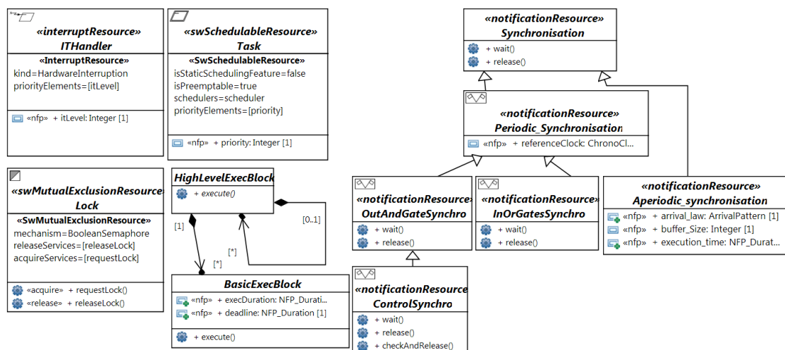
Figure 3 : Computational Model - MARTE::SRM Model
