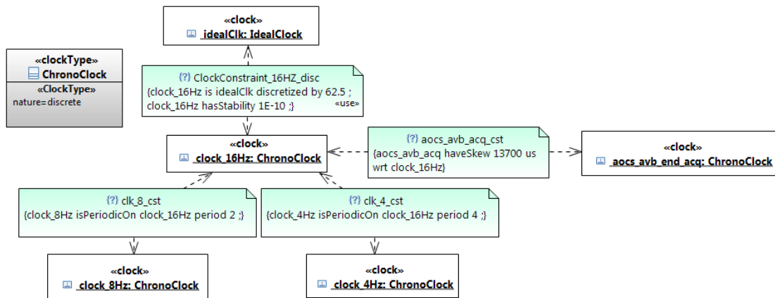
Figure 4 : Clocks definition
