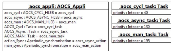
Figure 7 : Instance Diagram to specify the values of NFP
