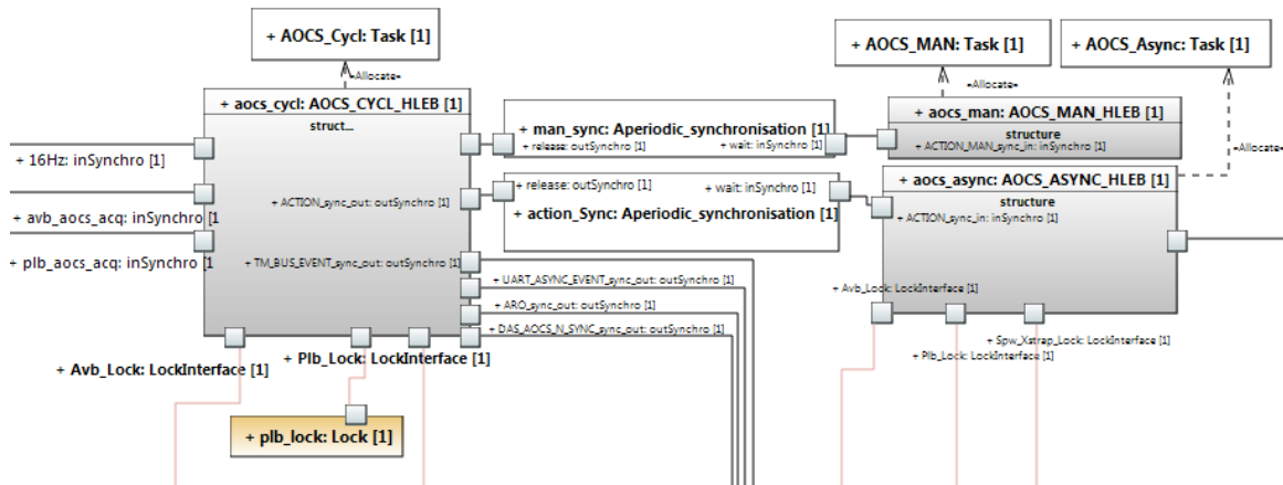
Figure 6 : Dynamic Architecture of AOCS_Appli (UML Composite Diagram)
