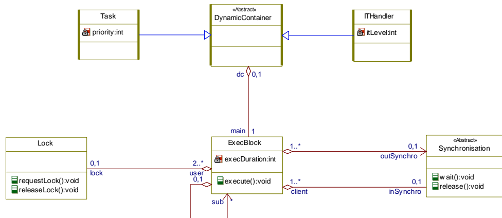
Figure 2 : Domain Model: Core Elements
