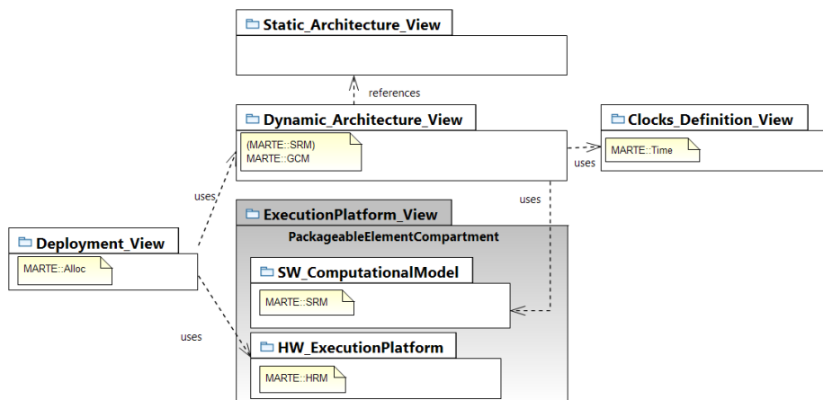
Figure 1 : Overview of the Modeling Methodology
