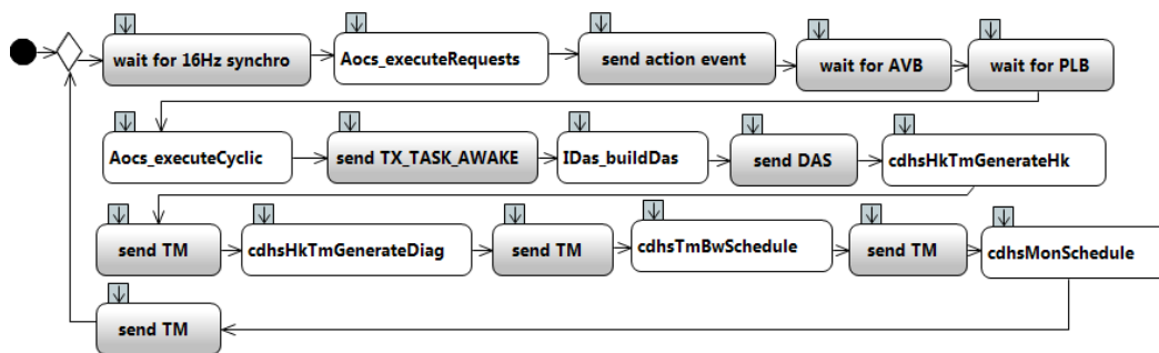
Figure 8 : Control Flow of AOCs_CYCL High Level Execution Block
