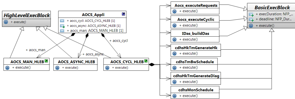
Figure 5 : Execution Blocks Definition (UML Class Diagram)
