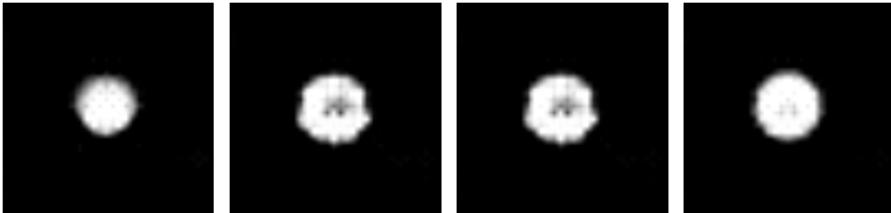
Regularisation type 3, \lambda = 10.0
