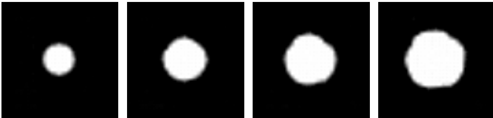
Regularisation type 3, \lambda = 50.0
