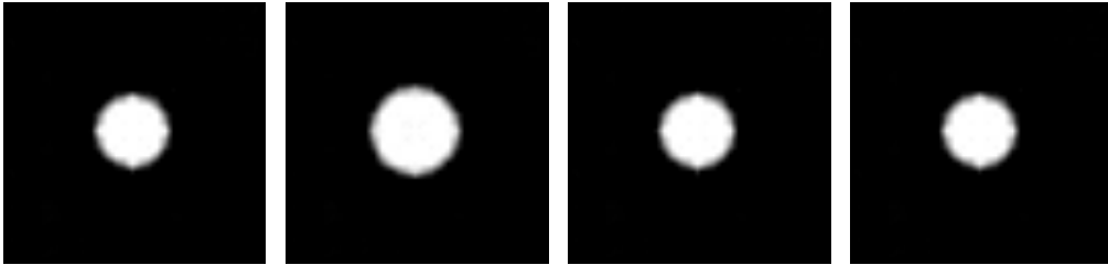
Regularisation type 3, \lambda = 1.0
