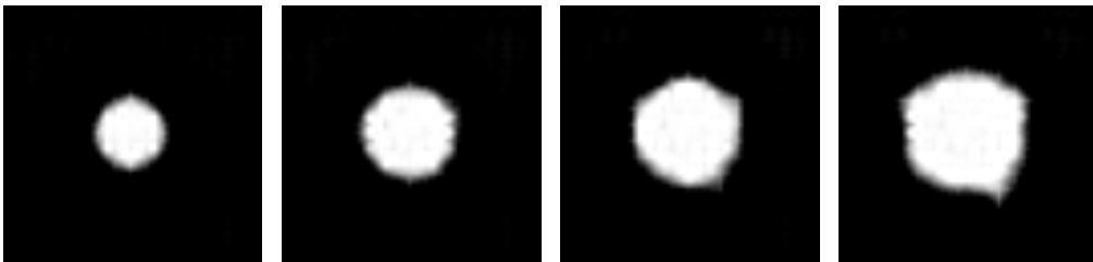
Regularisation type 3, \lambda = 100.0
