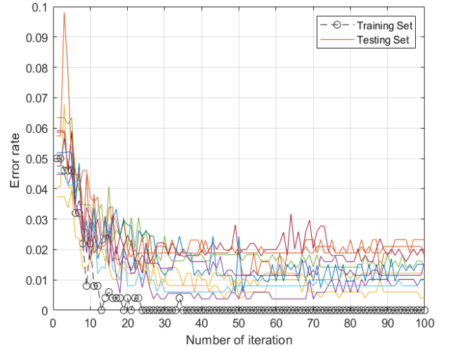
Fig. 5: Learning validation error.
