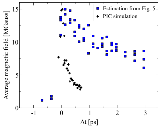
FIG. 7: Square: average magnetic field obtained from the ellipticity variation (figure 5a). The maximum magnetic field amplitude has been matched to PIC simulation results.
