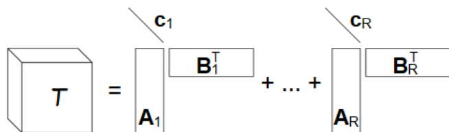
Fig. 1: Visual representation of BTD of an arbitrary third-order tensor.
