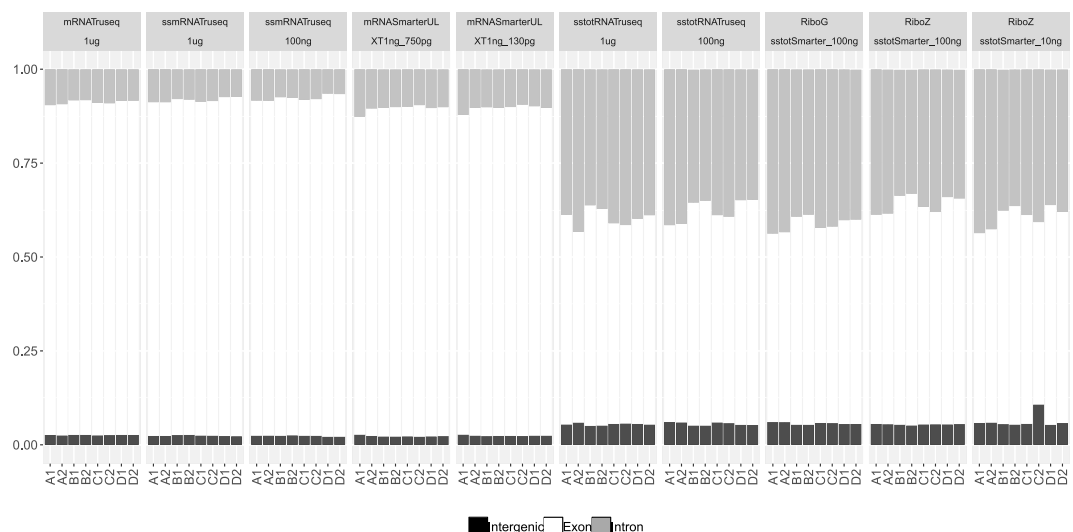
Figure 2. Normalized alignment rates (vertical axis) to intergenic, exon and intron regions for all the samples and conditions (horizontal axis). The mRNA samples are located on the left side of the figure and the total RNA samples are on the right side.
