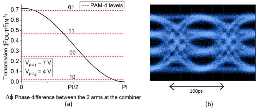
Figure 1. (a) Obtained PAM-4 levels by applying a 4-V peak-to-peak voltage on one arm and 7-V peak-to-peak voltage on the second arm on the silicon MZM numerical model. (b) Experimental eye diagram obtained after applying the same peak-to-peak voltages on the silicon MZM.
