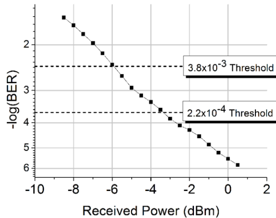
Figure 2. Measured O-band PAM-4 BER with the silicon MZM driven by a 7-V PP and a 4-V PP PRBS as a function of the received optical power.
