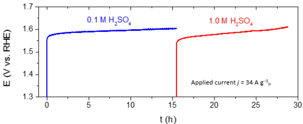
Figure S 11 Electrochemical stability of the \beta -H 2 IrO 3 catalyst. The electrode was applied with a constant current of 2 mA cm -2 oxide in O 2 -saturated 0.1 M H 2 SO 4 solution for 15 hours then in O 2 -saturated 1.0 M H 2 SO 4 solution for 14 hours.
