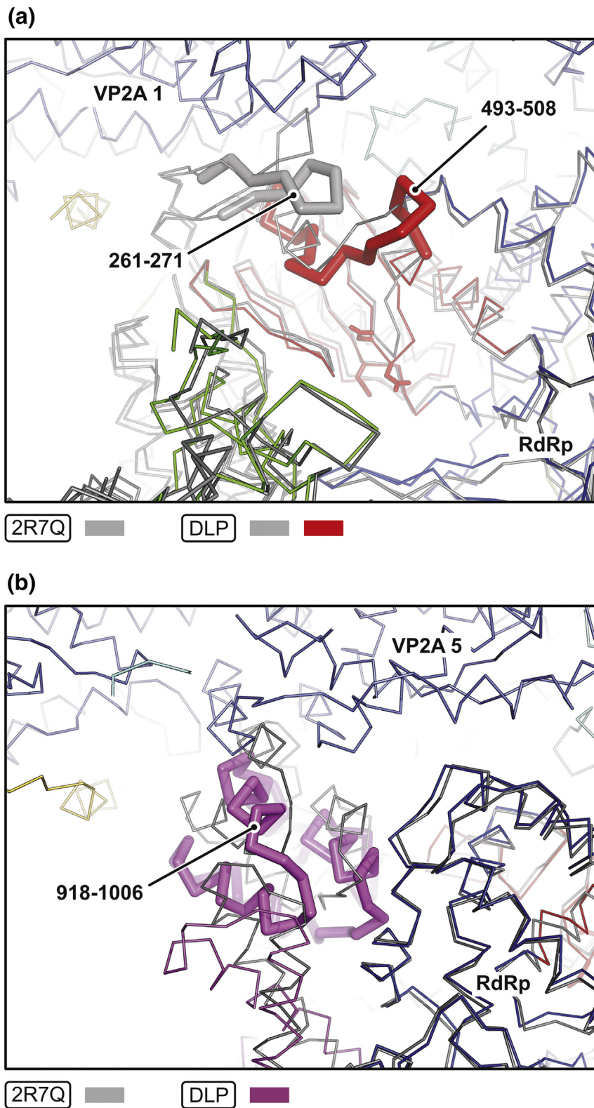
Fig. 4. Conformational changes between the VP1 crystal structure (RdRp in isolation, colored in gray, PDB-2R7Q) and our DLP structure (VP2-bound RdRp, colored as in Fig. 3). The two structures were superimposed using corresponding residues of the fingers, palm, and thumb domains only. (a) Close-up view showing the hairpin, residues 261–271, of the RdRp N-terminal domain, and the proposed “priming loop,” residues 493–508. RdRp active site residues are shown as sticks. For clarity, the bracelet domain is omitted. (b) Close-up view of the bracelet alpha-helical subdomain, residues 918–1006.
