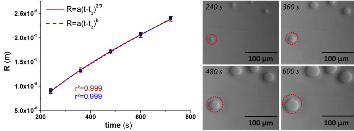
Fig. 3. Typical images of the dewetting on a PS film (260 nm) on top of PMMA (3 \mu m) at 200 ^{\circ} C at various times (right). The growth of the hole within the red circle is plotted as a function of time on the left. The red line represents the fit with the 2/3 dependence fixed. The blue line represents the best fit with the time dependence floating. (For interpretation of the references to colour in this figure legend, the reader is referred to the web version of this article.)
