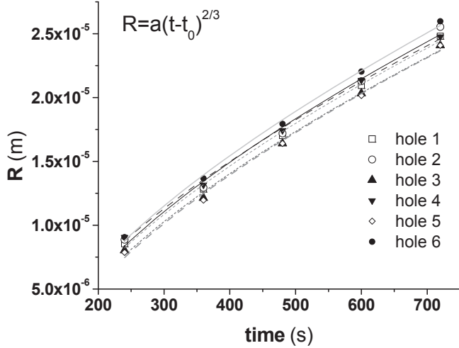
Fig. 4. Radius as a function of time for 3 holes on 2 different samples at the same experimental conditions ( T = 200 ^{\circ} C, d_{PS} = 260 nm, d_{PMMA} = 3 \mu m). Solid lines are fits following equation (4).
