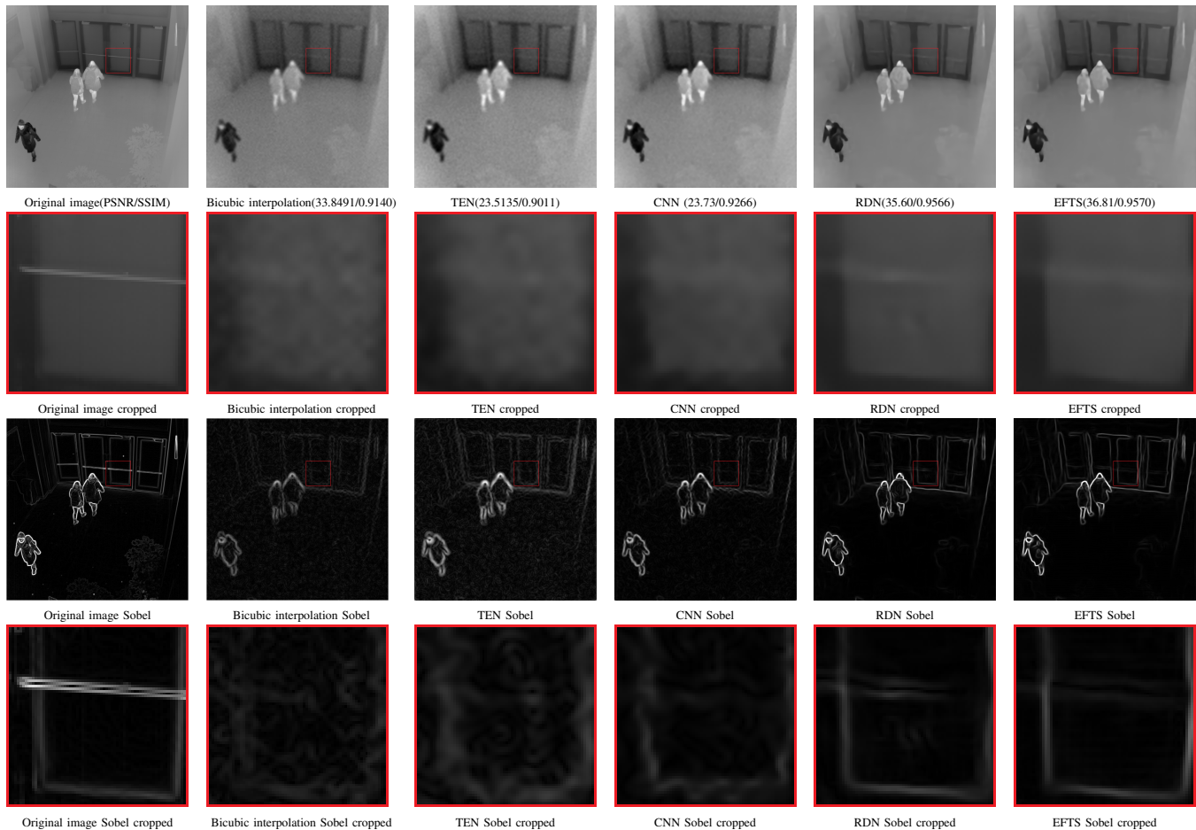
Figure 3: SISR using a blur kernel of 3 and a noise of 50
