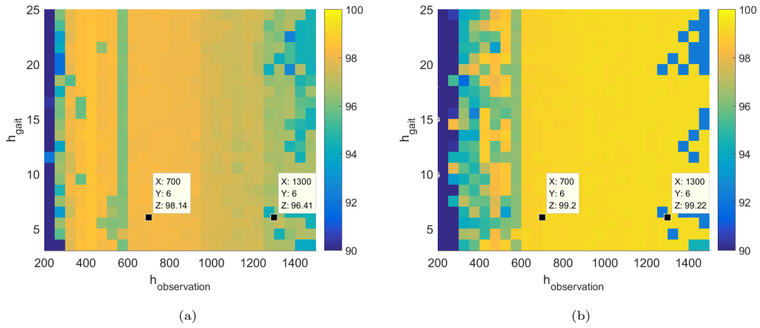
Figure 8: Averaged activity recognition accuracy (in %) according to h_{observation} and h_{gait} (size of stacks), for the first section of experiment (a) and for the second section (b).
