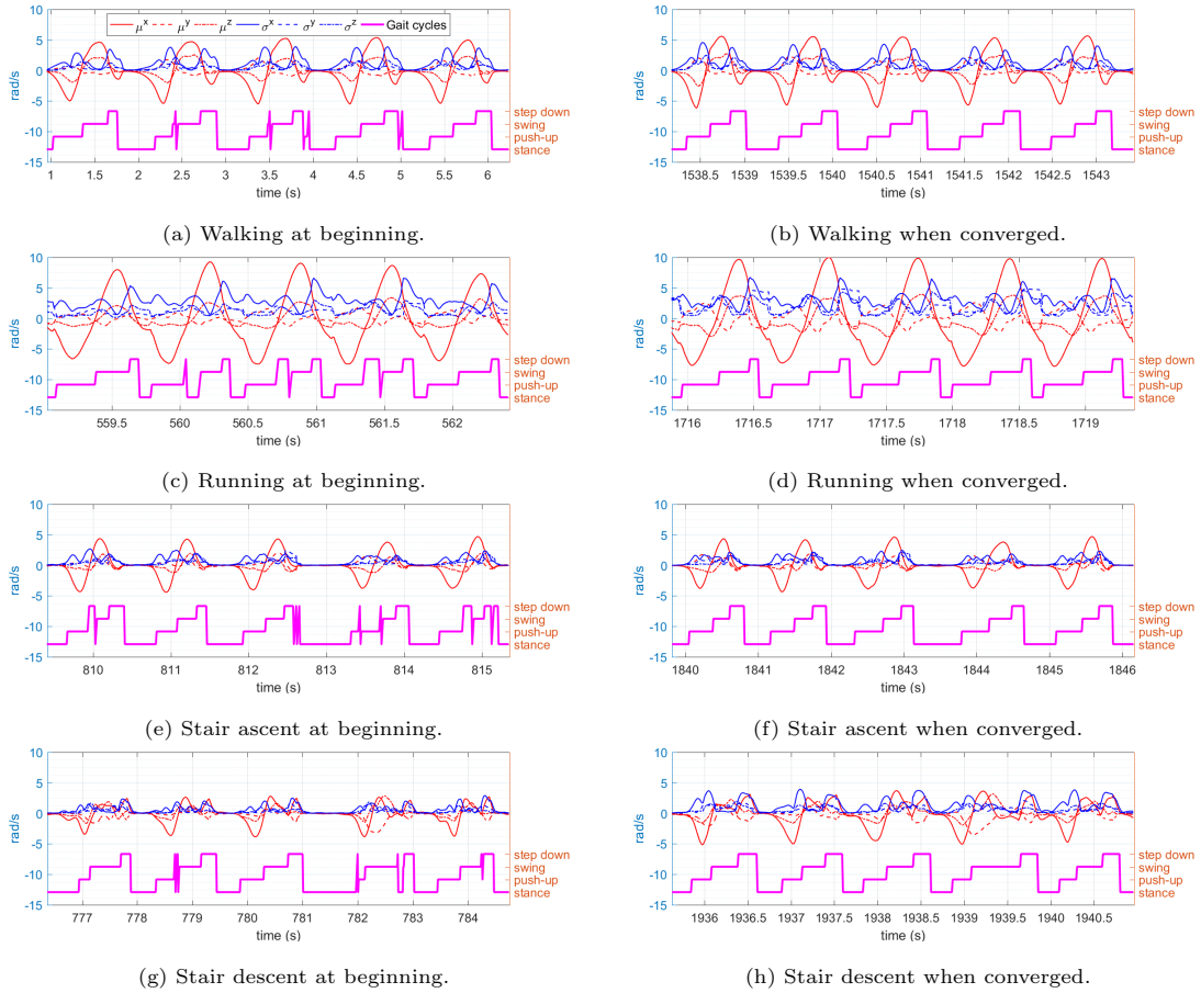
Figure 11: The detected gait cycles at the beginning of each activity (left column) compared to the ones when the estimation of the model's parameter has converged (right column).
