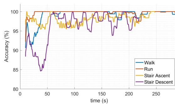
Figure 9: Accuracy in the most recent 1000 samples w.r.t. each activities.
