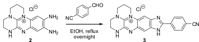
Scheme 4. Synthesis of diamino quinoxalium derivative 3 .
