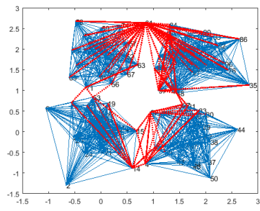
(b) Representation of R^{\varepsilon^*}
