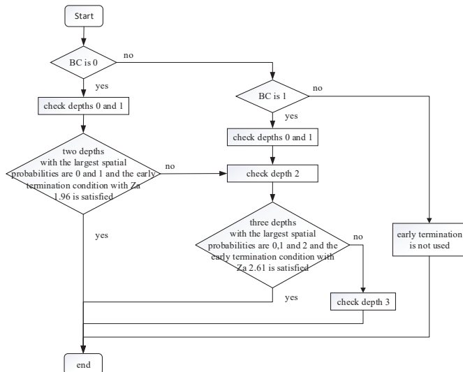
Fig. 8: Flowchart of the depth early termination
