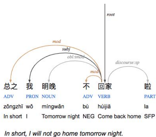
Figure 1 word-based treebank
