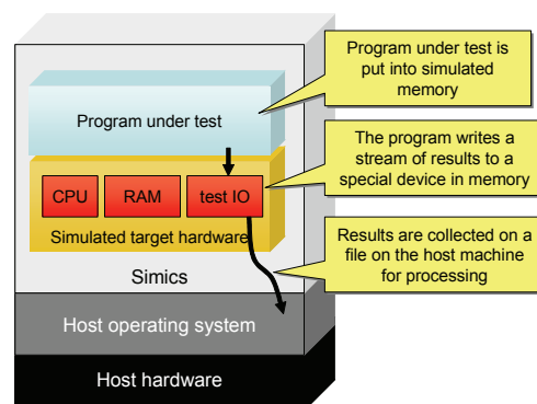
Figure 6: Setup for simple unit testing
