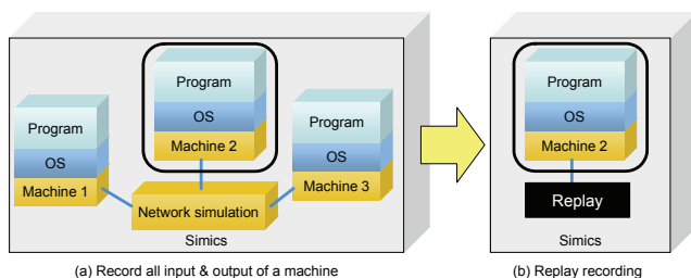
Figure 9: Record and replay in a network
