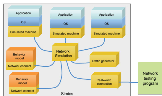
Figure 8: Network testing using a variety of simulation styles for different nodes
