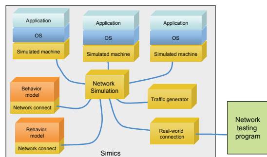
Figure 8: Network testing using a variety of simulation styles for different nodes
