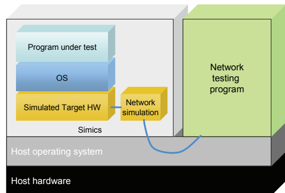
Figure 7: Network test on a single machine
