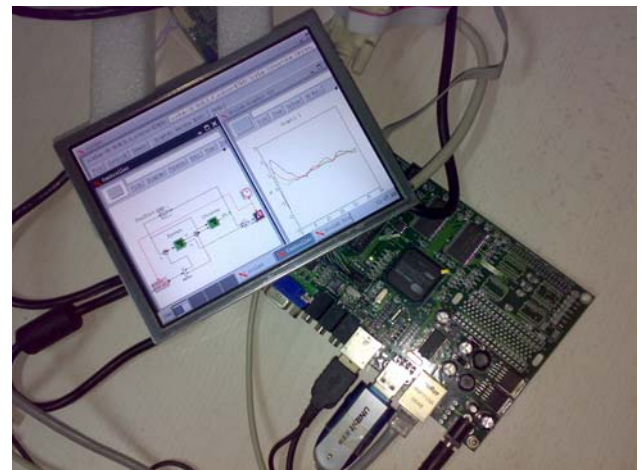
Figure 5: Scilab EMB.
