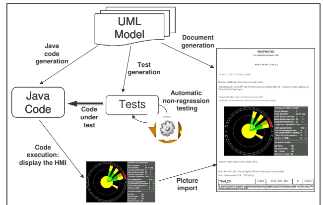
Figure 5: The MDE process for HMI
