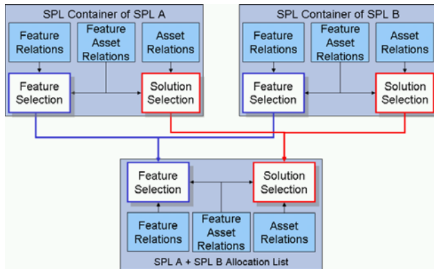
Figure 8: Allocation list
