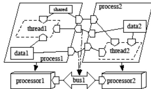
Figure 2: Architectural impact of the Bakery algorithm
