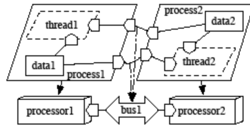
Figure 1: Data shared between two processes
