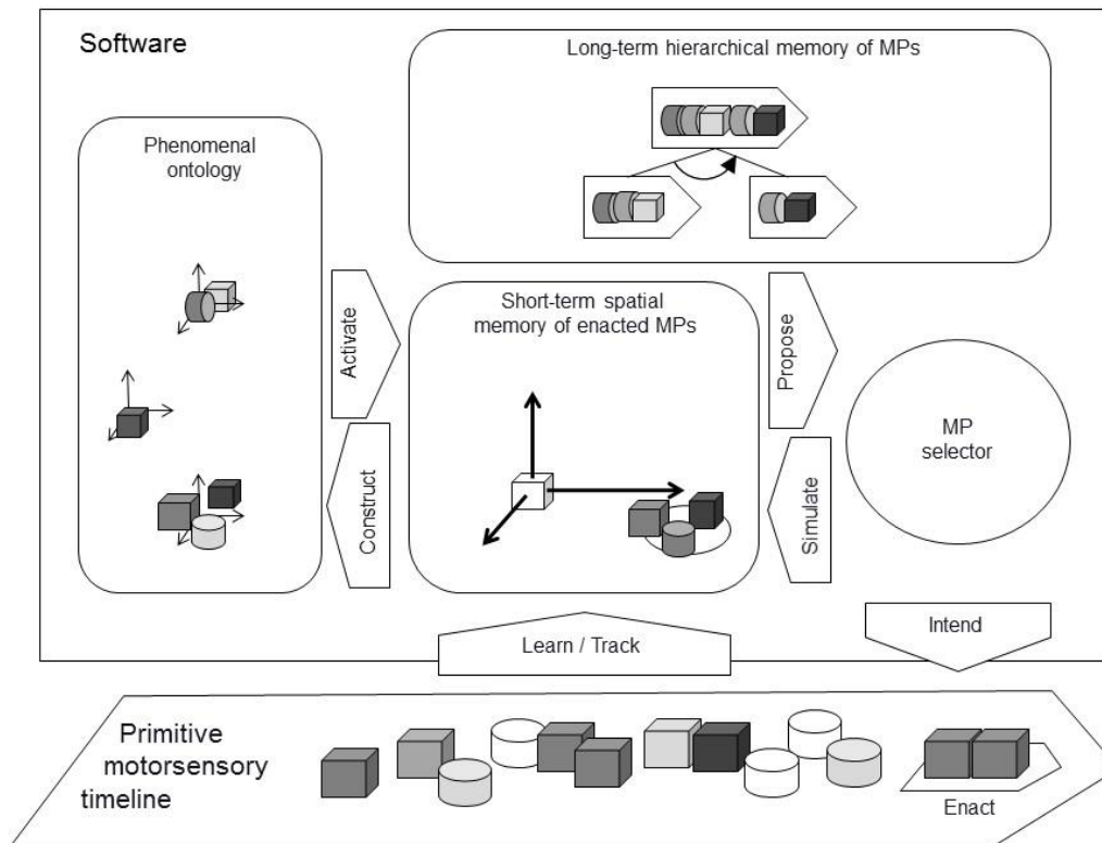
Figure 4. Spatio-temporal motorsensory cognitive architecture (adapted from Georgeon, Marshall & Manzotti 2013). Bottom: The primitive motorsensory timeline shows the stream of PMSs enacted over time. PMSs are represented as 3D cubes and cylinders to highlight that they specify the control of actuators with feedback within the presupposed 3D world. Top: The long-term hierarchical memory of MPs implements CASH. Center: The egocentric spatial memory tracks the position of enacted MPs relative to the entity over the short term. It is also used to simulate the enaction of future MPs before selecting them. Left: The phenomenal ontology records models of phenomena (spatio-temporal arrangements of MPs) constructed from spatial memory. Models of phenomena are how the software represents entities experienced in the 3D world (the entity that the software is controlling and other entities with which it is interacting). Activated instances of phenomena in spatial memory propose the MPs that they afford. Right: Selection of the next MP to try to enact in the environment.
