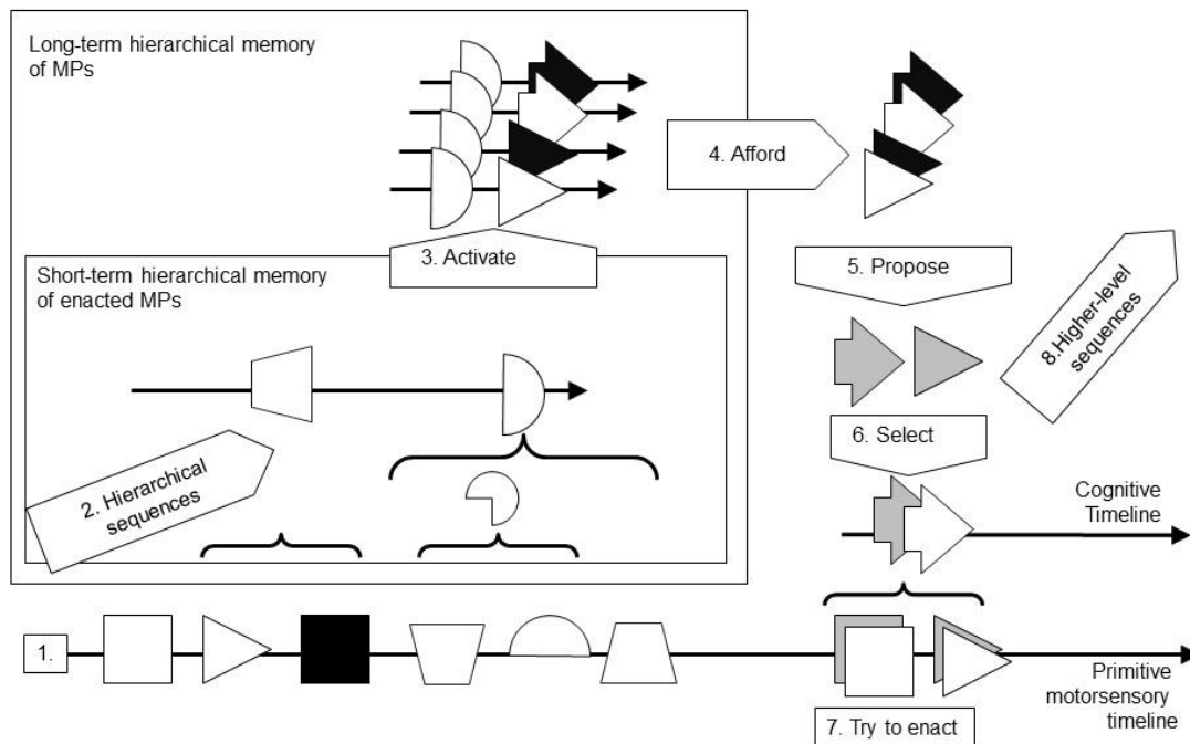
Figure 2. The MP learning and selection. 1) The primitive motorsensory timeline shows the series of PMSs enacted over time represented by geometrical shapes. 2) The short-term memory of enacted MPs shows the hierarchy of MPs that have been just enacted. 3) An MP represented by a half-circle activates several previously-learned higher-level MPs (stored in long-term memory) that begin with this MP. 4) Activated MPs generate a set of afforded MPs that consist of continuing to enact the activated MPs. 5) Afforded MPs are categorized in possible cognitive actions (gray shapes). 6) The cognitive timeline shows selected MPs and enacted MPs passed through the cognitive coupling. Based on possible cognitive actions, the software selects an MP to try to enact (Gray arrow on the cognitive timeline). 7) The entity tries to enact the PMSs that constitute the selected MP and returns the enacted MP (white arrow). 8) Higher-level MPs can be learned on the basis of enacted MPs.
