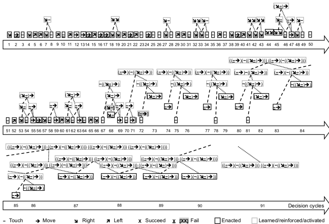
Figure 3. Demonstration of motorsensory self-programming (Georgeon & Ritter 2012). The agent has three possible output values corresponding to touch front , step forward , turn right , turn left and a single bit input value, forming 6 PMSs. Over time, a hierarchy of MPs is learned from the bottom up in a pairwise manner. Various two-step MPs are enacted during cognitive cycle 44, 45, 68, 74. A six-step MP is enacted four times in a row during cognitive cycles 87, 88, 89, 90. It consists of the sequence: touch front nothing – step forward – touch front something – turn right – touch front nothing – step forward . This MP captures a regularity afforded by the agent–environment interactional domain consisting in turning around in a box without bumping into the walls.
