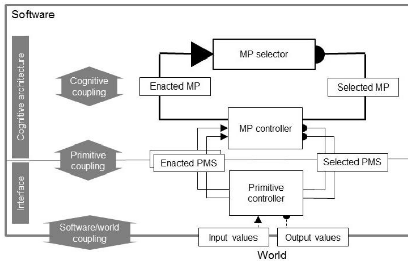
Figure 1. The software implemented in the entity. The large gray frame (software/world coupling) delineates the software coupled with the world (entity + environment) through the output and input registers. The light gray line (primitive coupling) delimits the cognitive architecture (above) from the interface (below). The interface controls the enaction of primitive motorsensory schemes (PMS) through motor commands and sensor feedback, and then returns the enacted primitive motorsensory schemes. The cognitive coupling links the motorsensory process selector (above) with the motorsensory process controller (below) responsible for sequentially sending the selected primitive motorsensory schemes to the primitive controller. As the cognitive architecture learns higher-level MPs, one round of the cognitive coupling corresponds to several rounds of the primitive coupling.
