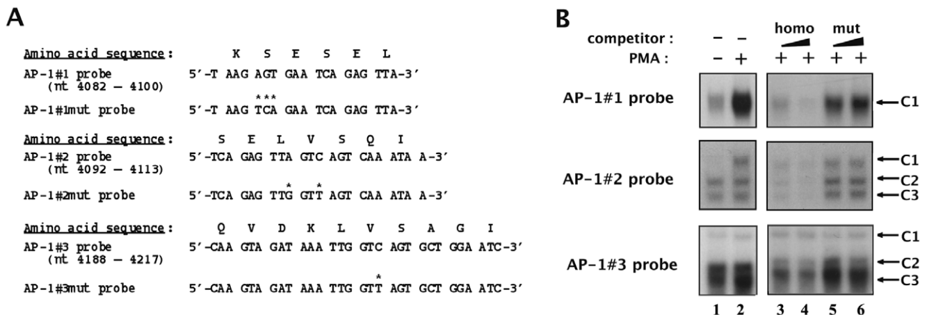
Figure 3. Identification of point mutations which abolish AP-1 transcription factors' in vitro binding to their respective binding sites located in fragment 5103. (A) The wild-type and mutated AP-1#1, AP-1#2 and AP-1#3 oligonucleotide sequences are indicated as well as the corresponding underlying amino acid sequence of the viral reverse transcriptase. Base pairs which were modified in the mutated versions of the AP-1 binding sites relative to the wild-type versions are indicated by asterisks. (B) The AP-1#1, AP-1#2 and AP-1#3 oligonucleotide probes were incubated with nuclear extracts (10 µg) from mock-treated (lane 1) or PMA-treated (lanes 2 to 6) HeLa cells in the absence of competitor (lanes 1 and 2) or in the presence of increasing molar excesses (2 and 4 fold) of each respective homologous AP-1 oligonucleotide (lanes 3 and 4) or of the corresponding mutated AP-1 oligonucleotide (lanes 5 and 6). The figure shows the specific retarded bands of interest, which are indicated by arrows. doi:10.1371/journal.pone.0019084.g003
