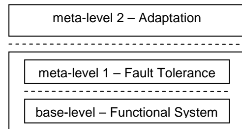
Figure 1 : Reflective architecture
