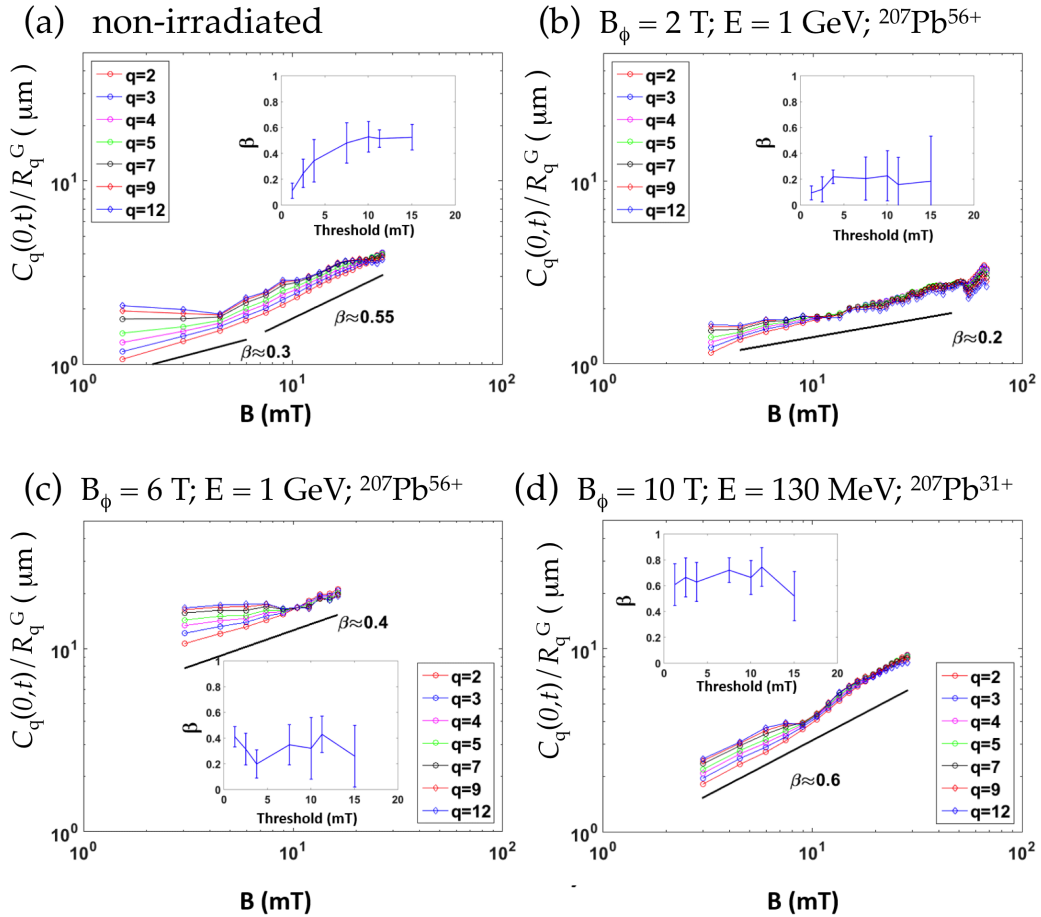
Figure 7. Main panels: “Temporal” correlation functions C_q(0, t) describing the growth of flux front features as the magnetic flux advances from the chemically etched boundaries of films Y0T (a), Y2T (b), Y6T (c), and Y10T (d). The insets show the growth exponent \beta , as extracted from the lowest order C_2(0, t) , as function of B_t .
