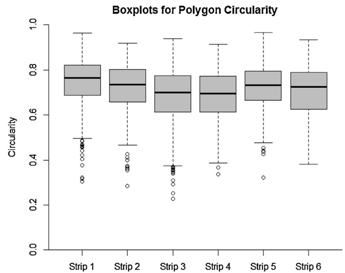
Fig. 18. Boxplots displaying polygon circularity values for all of the strips analysed. The boxes represent the interquartile range of each strip. The bold horizontal line is the median of each strip. The whiskers represent the upper and lower quartile. The outliers are located 1.5 times the interquartile range above the upper quartile.
