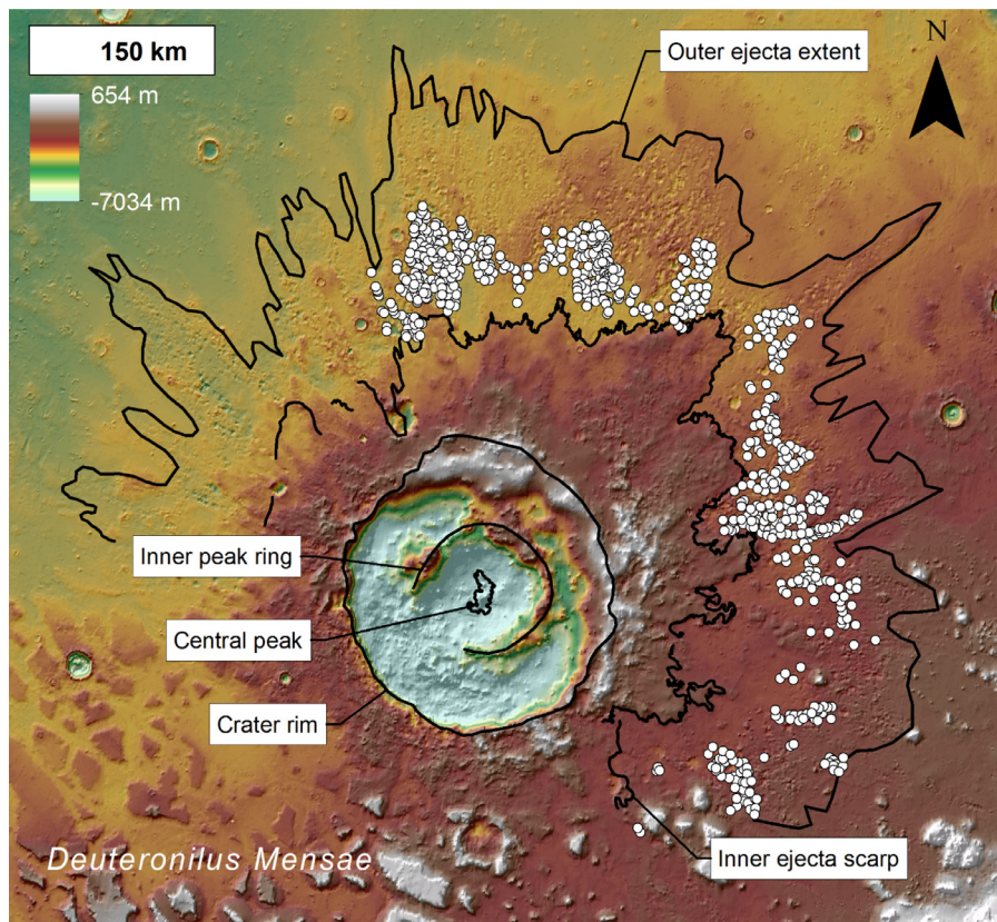
Fig. 2. Lyot crater study area displayed using coloured Mars Orbiter Laser Altimeter (MOLA; Zuber et al., 1992) topographic data overlain on a MOLA hillshade. The crater peak, inner peak ring, crater rim, inner ejecta scarp and outer ejecta extent are indicated by black lines. Regions of clastic polygonal features are marked as white circles. Image credit: MOLA Science Team.
