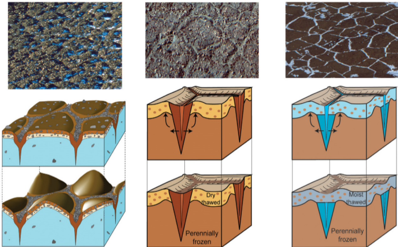
Fig. 5. Figure adapted from Fig. 6, Marchant and Head (2007). A) (Top to bottom) shows a photograph of sublimation polygons from the Antarctic Dry Valleys (FOV ~50 m) and a block diagram indicating how they might develop. B) (Top to bottom) shows a photograph of sand-wedge polygons from the Antarctic Dry Valleys (FOV ~100 m) and a block diagram indicating how they might develop. C) (Top to bottom) shows a photograph of ice-wedge polygons from the Antarctic Dry Valleys (FOV ~50 m) and a block diagram indicating how they might develop.
