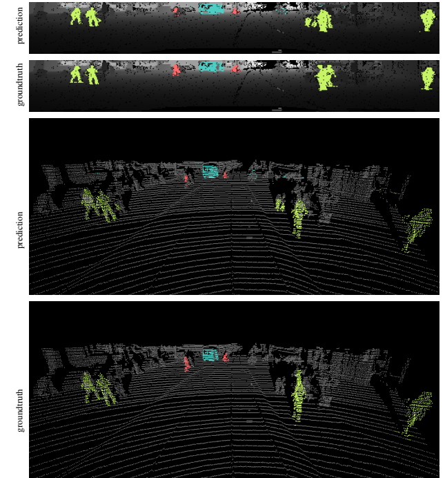
Figure 1. The two top first images show the segmentation of LiDAR data obtained with our method, and the groundtruth segmentation, seen in the sensor topology. The two bottom images show the same segmentations from a different point of view.
