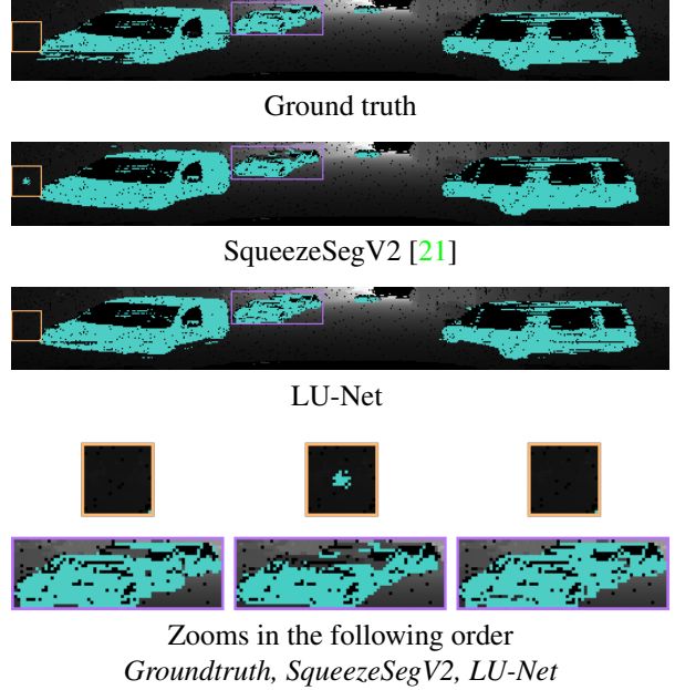
Figure 7. Visual comparison of the proposed model against SqueezeSegV2 [21] and the ground truth. Results are shown on the range-image where depth values are encoded in grayscale map. Both SqueezeSegV2 and LU-Net globally achieve very satisfying results. Nevertheless, LU-Net is less subject to false-positive compared to SqueezeSegV2, as can be seen in the orange areas and corresponding zooms. It also better segments farther objects such as the cars on the back of the scene in the purple rectangle, which reduces the amount of false-negative, which are crucial for autonomous driving applications.
