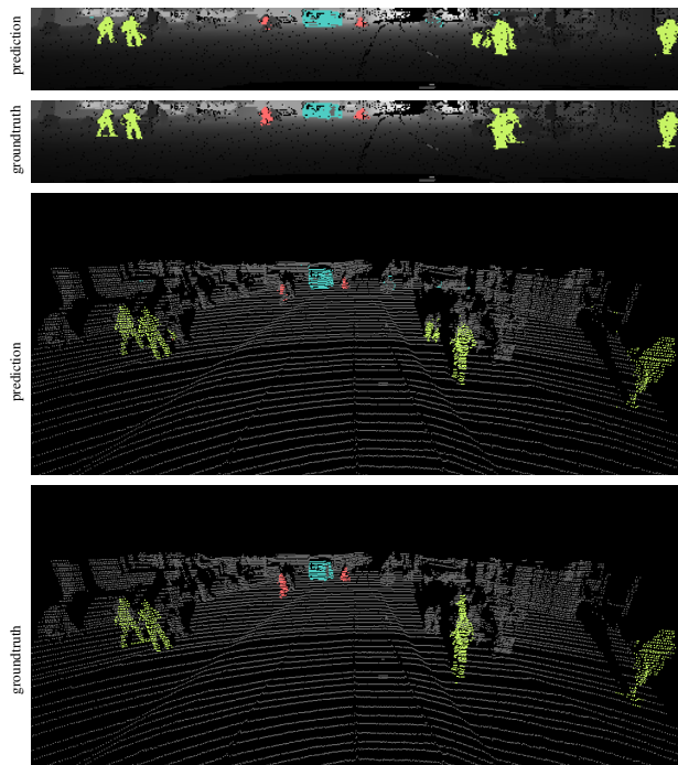
Figure 1. The two top first images show the segmentation of LiDAR data obtained with our method, and the groundtruth segmentation, seen in the sensor topology. The two bottom images show the same segmentations from a different point of view.
