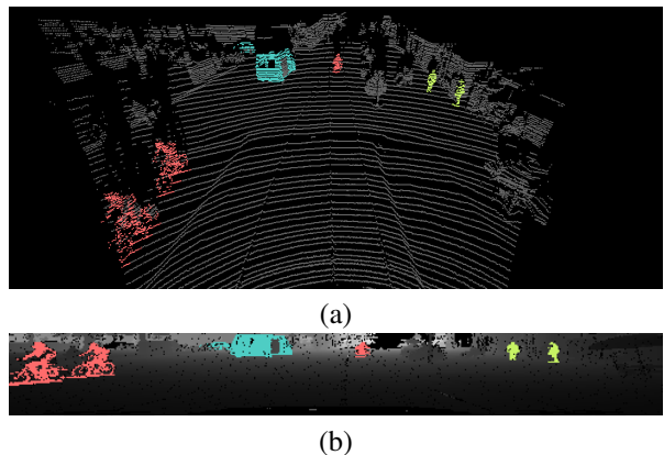
Figure 3. Example of a point cloud from the KITTI database [7] (a) turned into a range-image (b). Note that the dark area in (b) corresponds to pulses with no returns. Colors correspond to groundtruth annotation, for better understanding.
