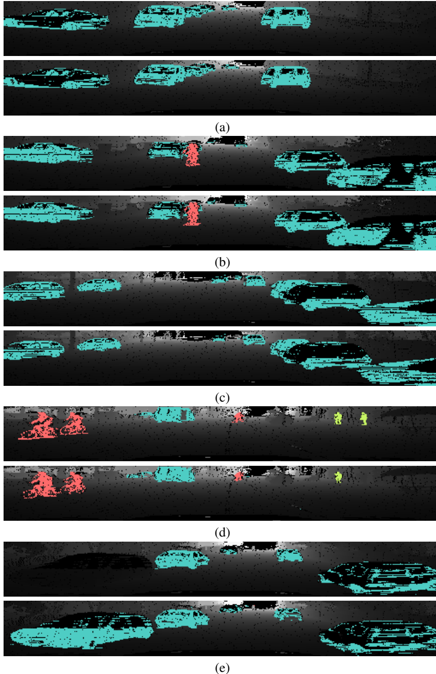
Figure 9. Results of the semantic segmentation of the proposed method (bottom) and groundtruth (top). Results are shown on the range-image where depth values are encoded in grayscale map. Labels are associated to colors as follows: blue for the cars, red for the cyclists and lime for the pedestrians.
