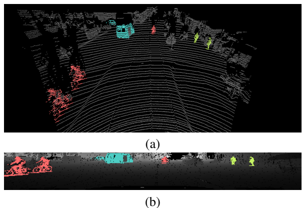
Figure 3. Example of a point cloud from the KITTI database [7] (a) turned into a range-image (b). Note that the dark area in (b) corresponds to pulses with no returns. Colors correspond to groundtruth annotation, for better understanding.
