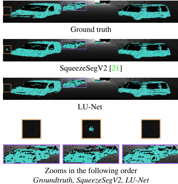
Figure 7. Visual comparison of the proposed model against SqueezeSegV2 [21] and the ground truth. Results are shown on the range-image where depth values are encoded in grayscale map. Both SqueezeSegV2 and LU-Net globally achieve very satisfying results. Nevertheless, LU-Net is less subject to false-positive compared to SqueezeSegV2, as can be seen in the orange areas and corresponding zooms. It also better segments farther objects such as the cars on the back of the scene in the purple rectangle, which reduces the amount of false-negative, which are crucial for autonomous driving applications.
