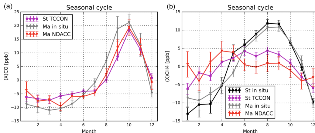
Figure 5. The seasonal cycles of CO (a) and CH 4 (b) from in situ and FTIR (NDACC and TCCON) measurements at St Denis and Maïdo. The error bar is 1 \sigma for all of the detrended data within that month.
